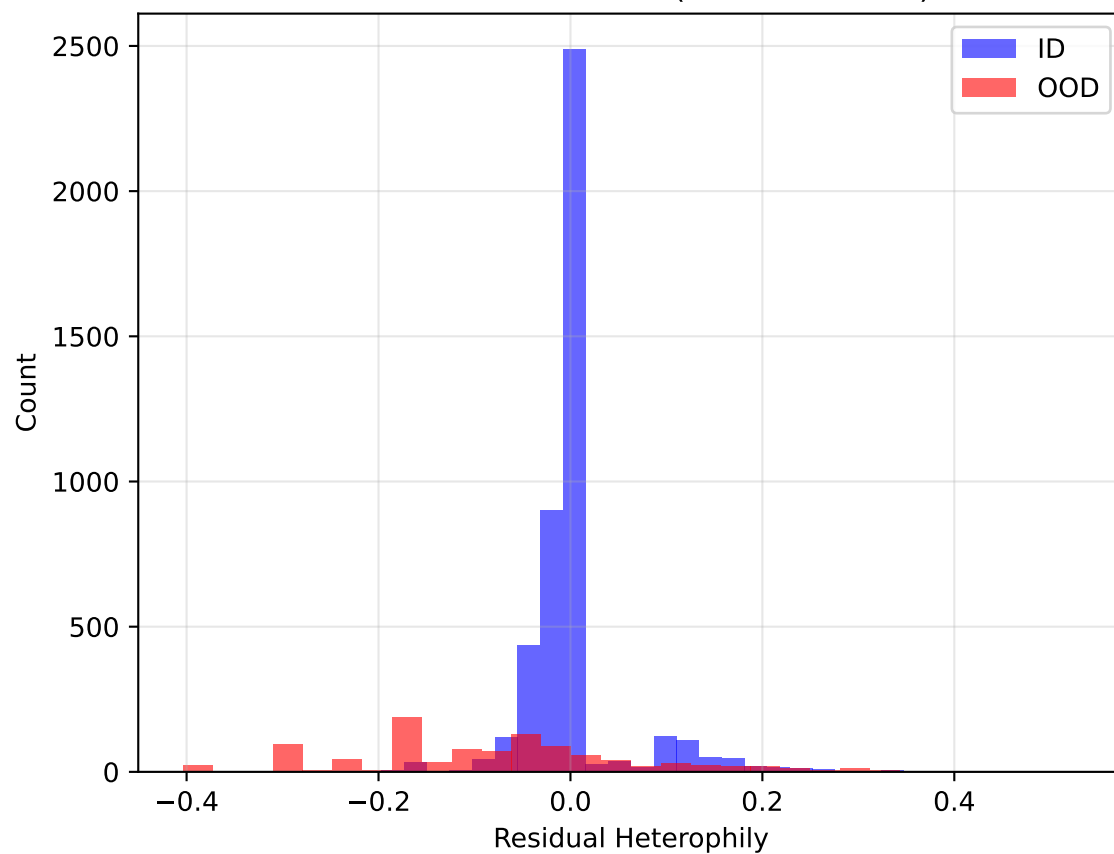
Residual Distribution (AUROC=0.272)
