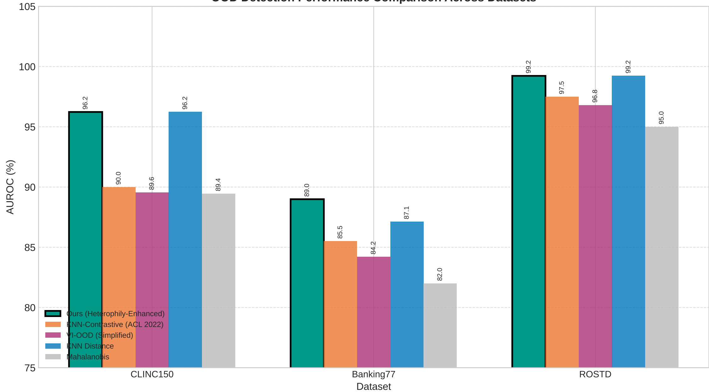
OOD Detection Performance Comparison Across Datasets
