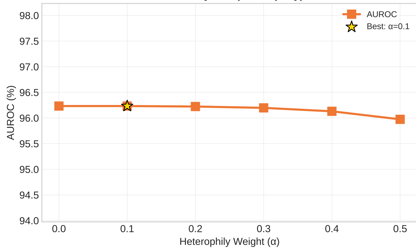
Sensitivity to \alpha (Heterophily)
