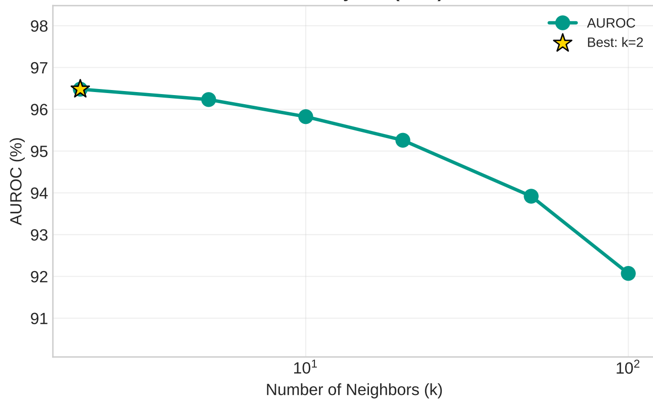
Sensitivity to k (KNN)
