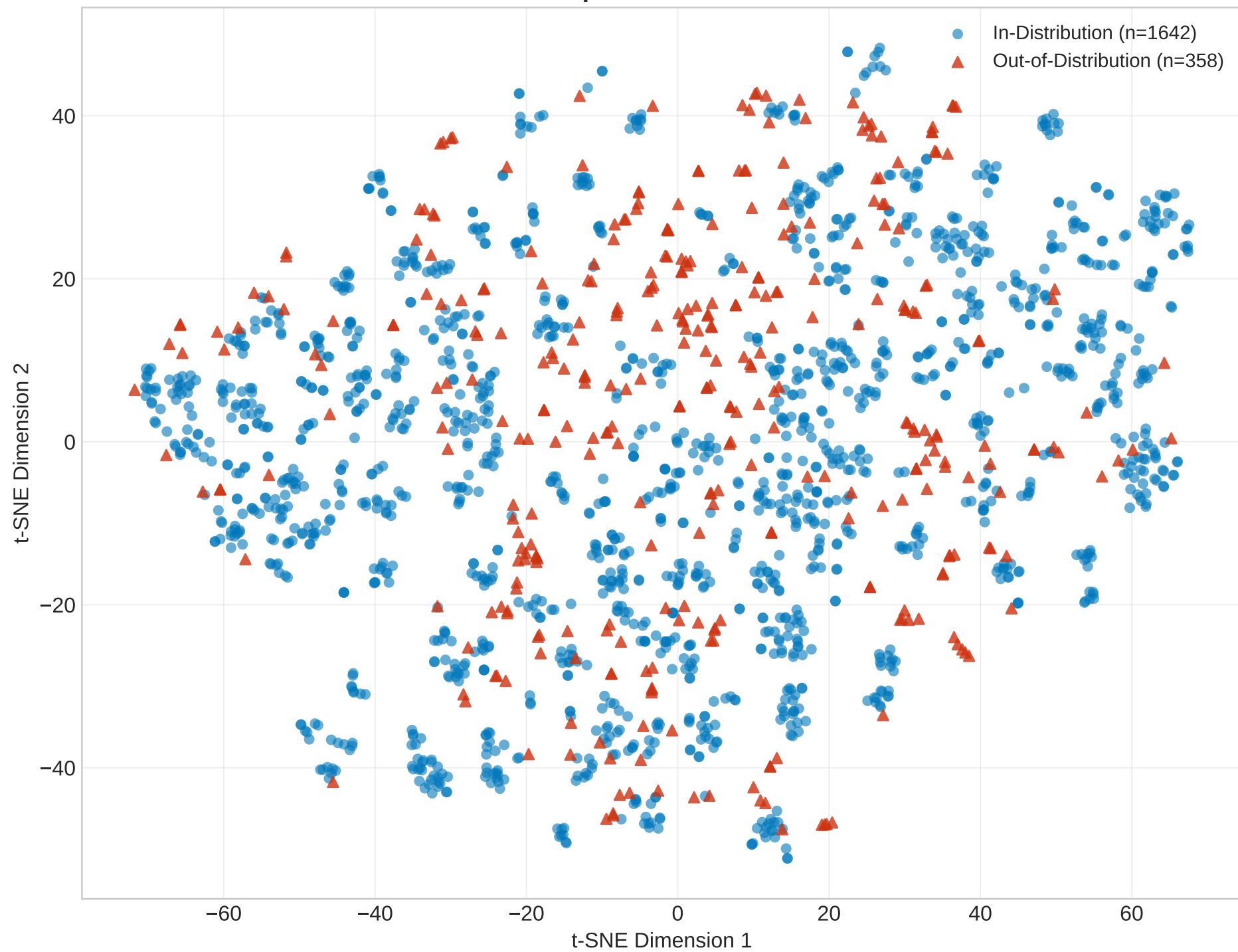
t-SNE Feature Space Visualization: CLINC150
