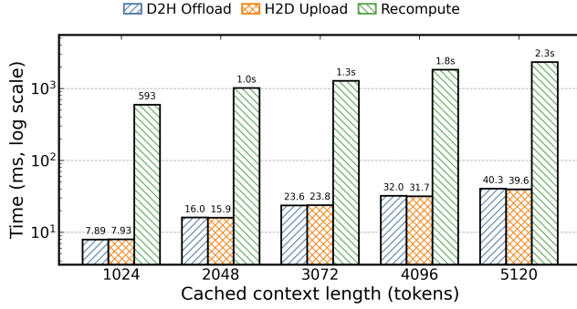
Figure 16. D2H offload, H2D upload, and recomputation time for Qwen2.5-14B on A100 PCIe.
