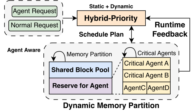
Figure 8. The Spatial Scheduler’s dynamic memory partitioning feedback loop.
