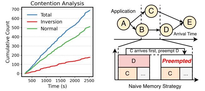
(a) Preemption events over time of the Code Writer workload. (b) KV Cache blocks held by non-critical agents.
