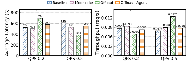
Figure 12. Mooncake comparison at 0.2 and 0.5 QPS.
