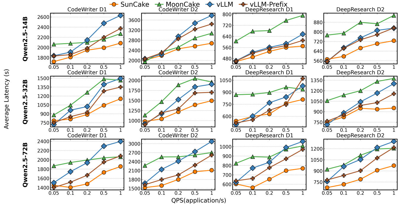
Figure 9. End-to-end application latency comparison of SunCake, vLLM, and Mooncake. Each chart plots average latency against queries-per-second (QPS) for the specified application, model, and dataset.
