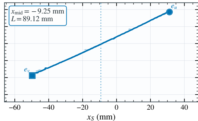
(c) After translation-servo correction
