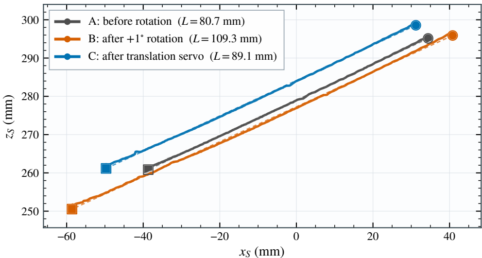
Measured plate-profile evolution in \{S\}
