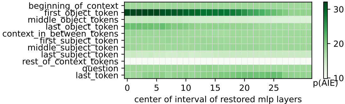
Impact of restoring mlp after corrupted input
