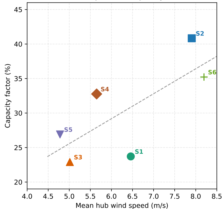
(a) Wind speed vs capacity factor
