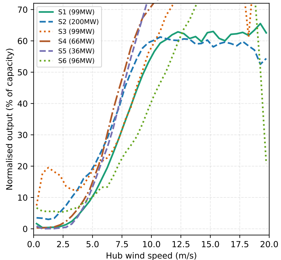
(c) Normalised power curves
