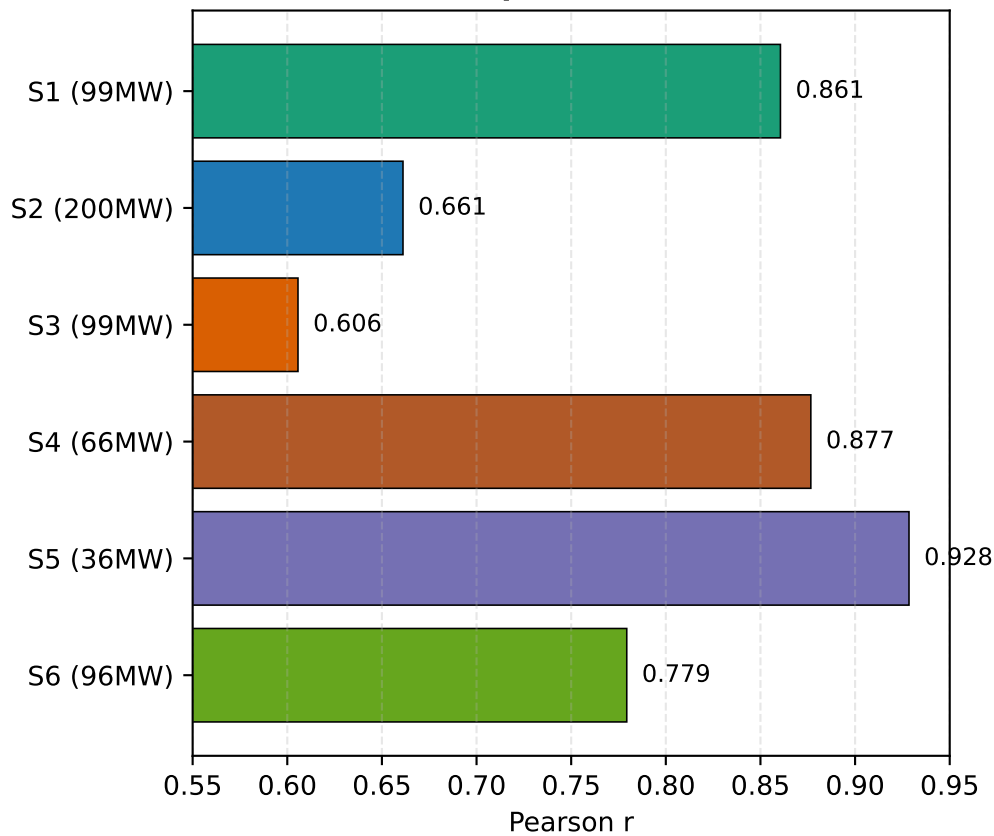
(b) Wind-power correlation
