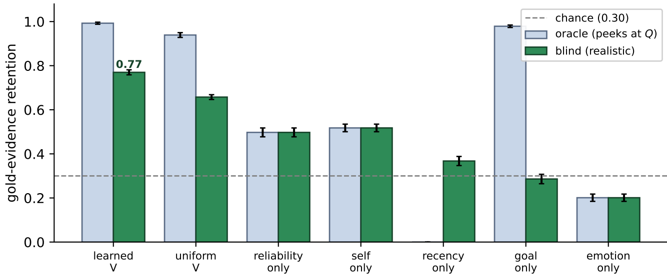
Blind vs. oracle forgetting (keep 30%, 479 cases, 20 splits; mean \pm 1 std)
