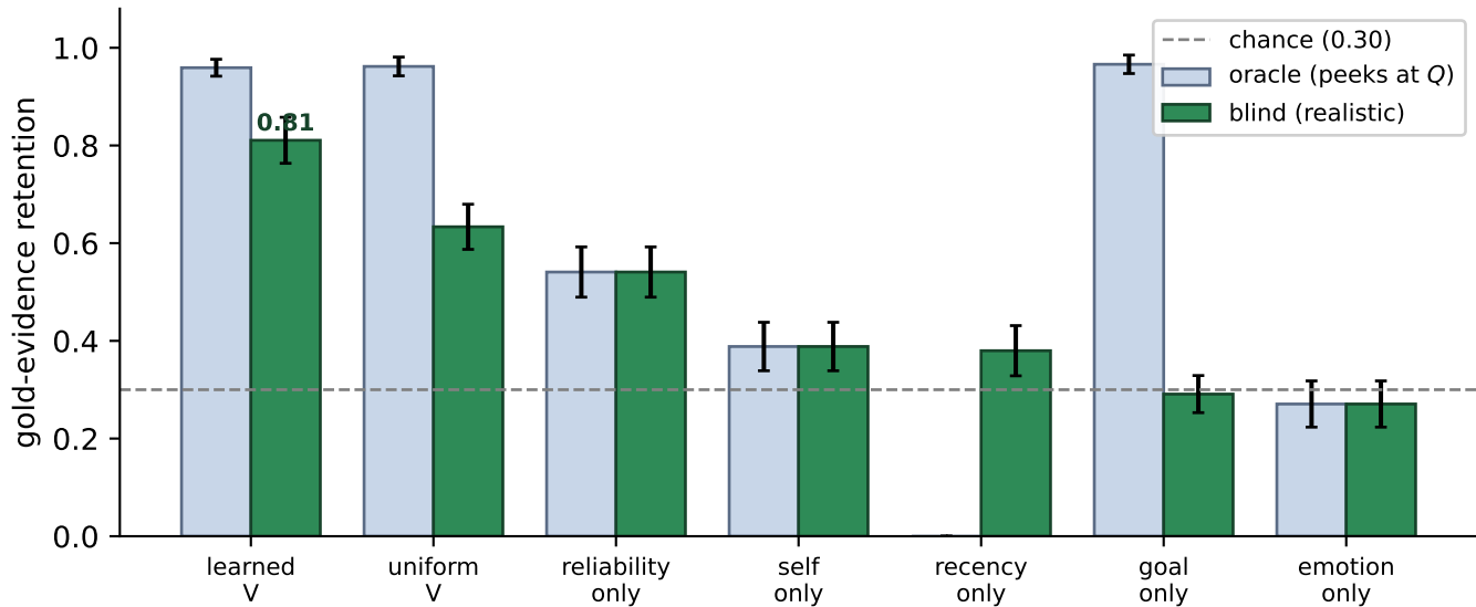
Blind vs. oracle forgetting (keep 30%, 74-case pilot, 20 splits; mean \pm 1 std)
