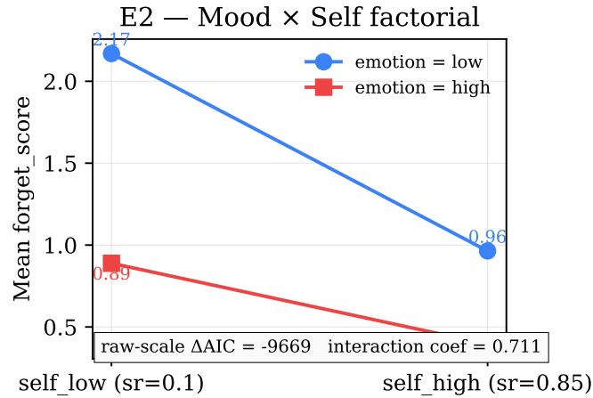
Figure 2: E2 — Mood \times Self factorial. Mean forget_score per cell. Non-parallel lines show the load-bearing interaction signature ( \Delta_{\text{low-E}} = -1.21 , \Delta_{\text{high-E}} = -0.49 ). OLS recovers the analytic \beta_{ES} = +0.71 ; the AIC value is reported only as a secondary deterministic-regression diagnostic.
