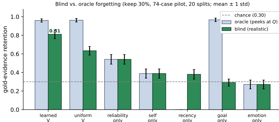
Figure 2: Blind vs. oracle gold retention (keep 30%; 74-case LongMemEval-S pilot; 20 resampled splits, mean \pm 1 std). Under the oracle goal anchor (cosine to the held-out question), similarity alone saturates retention — a retrieval ceiling. Under the realistic blind anchor (session topic only), every single-factor and recency baseline collapses toward the chance floor, while the learned multi-factor value retains 0.81. Recency has no oracle variant.
