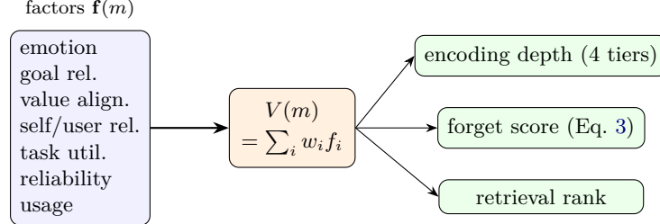
Figure 1: One value, three operations. A single learned scalar V(m) = \sum_i w_i f_i(m) over seven factors drives encoding depth, forgetting, and retrieval, replacing three separately tuned rules. The weights w_i are fit to a downstream objective (section 3.3).
