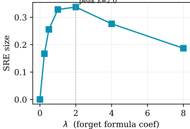
E3b — \lambda sensitivity (secondary)
