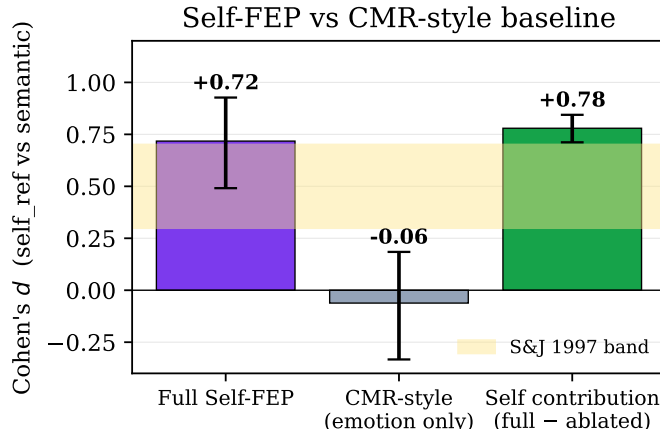
Figure 6: Head-to-head: Self-FEP vs CMR-style emotion-only baseline. Cohen's d with bootstrap 95% CI across 10 seeds. Removing the self component (centre bar) collapses the SRE; the self-contribution gap (right bar) has a CI that excludes zero and accounts for the entire observed effect.
