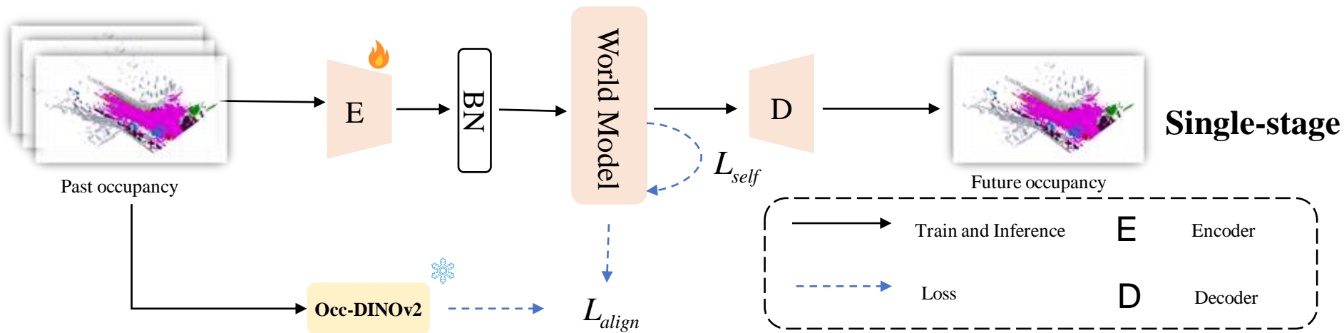
(b) E2EOcc: End-to-End 4D Occupancy World Modeling
