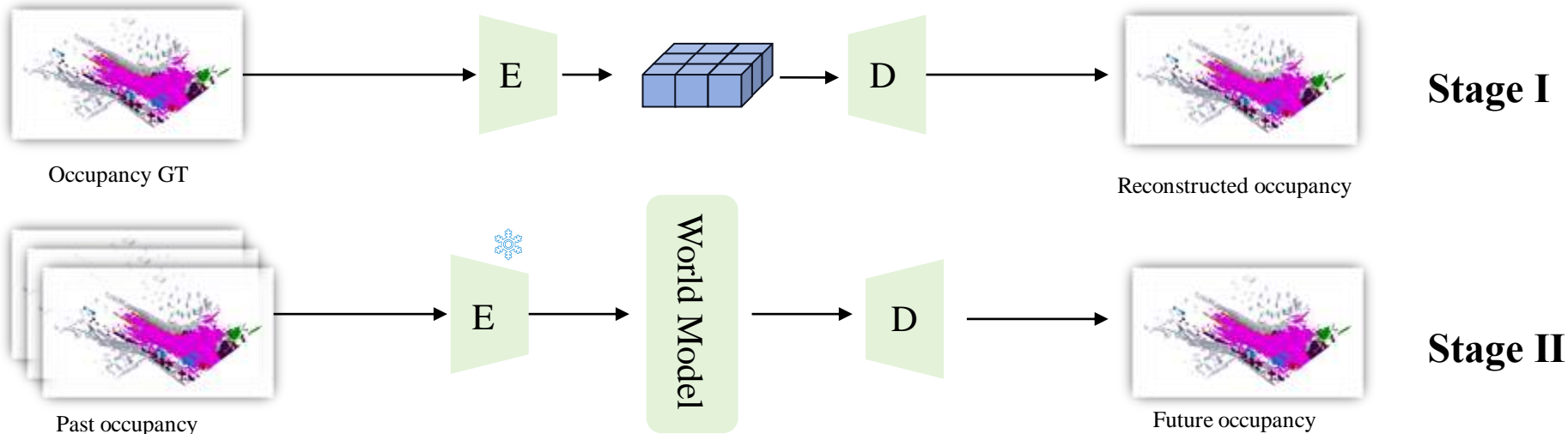
(a) OccSora: Two-stage training and autoregressive inference
