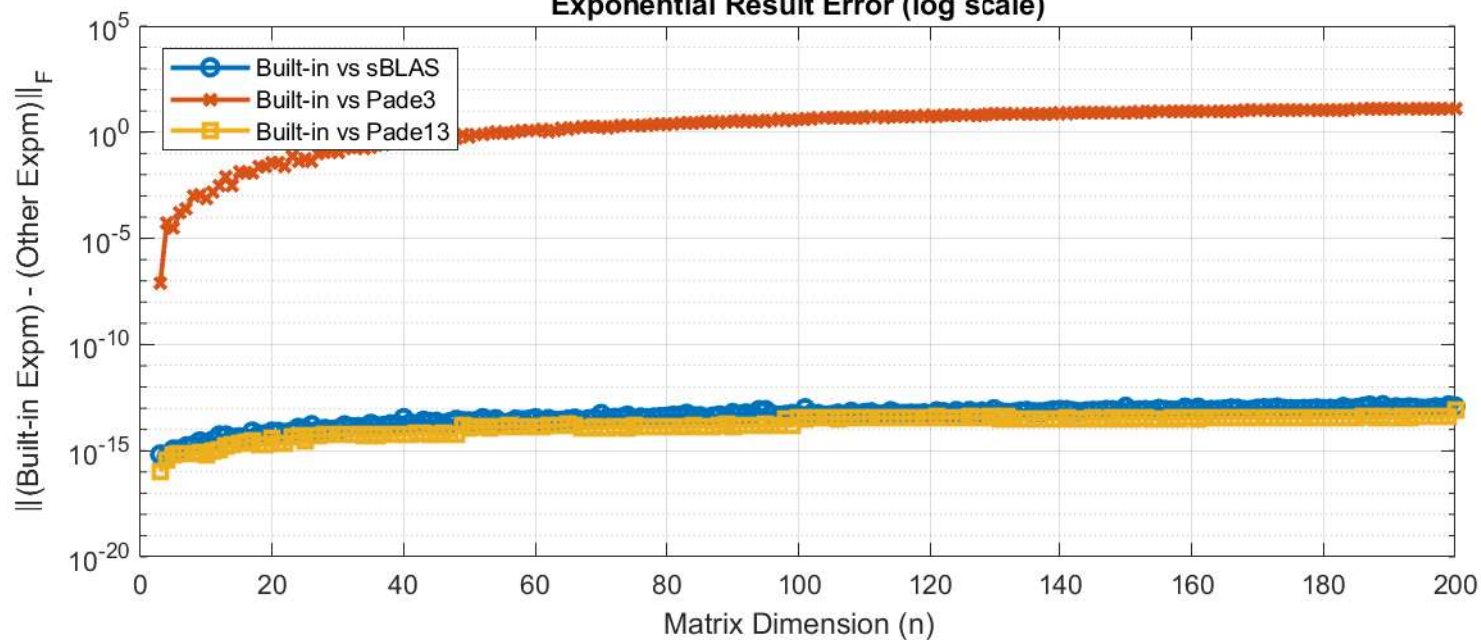
Exponential Result Error (log scale)
