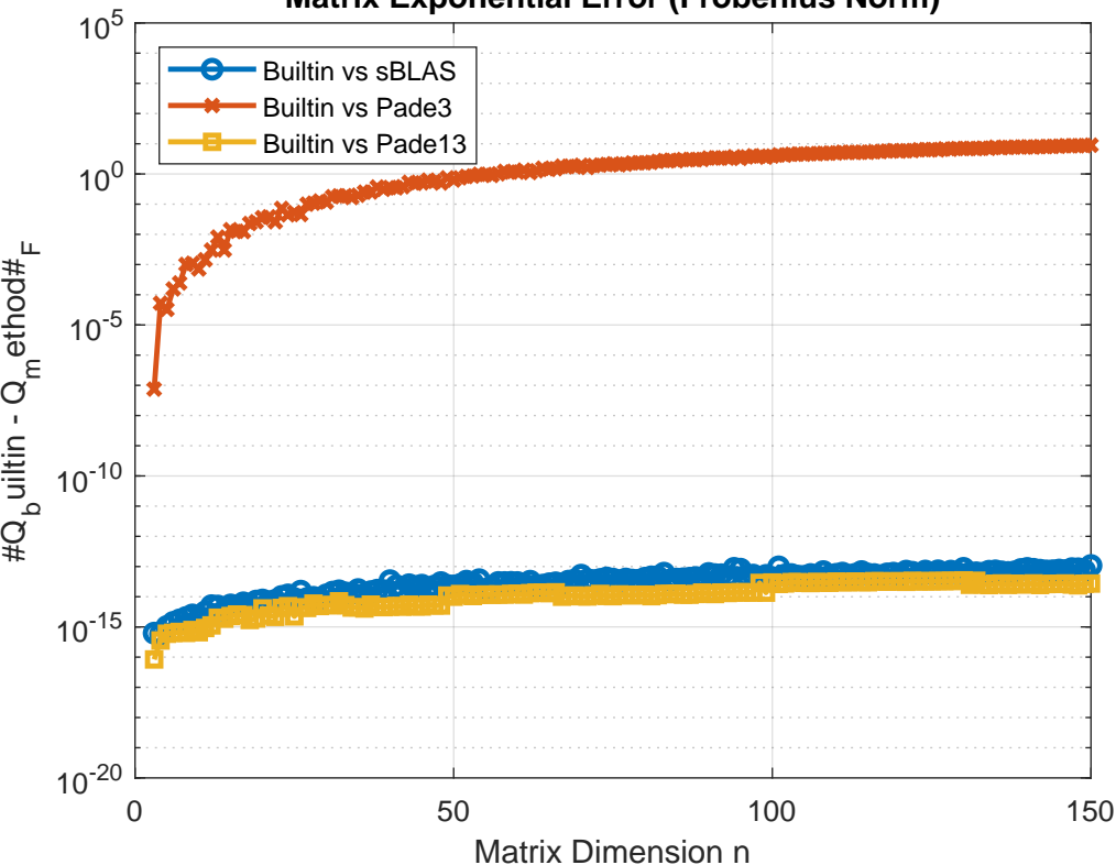
Matrix Exponential Error (Frobenius Norm)
