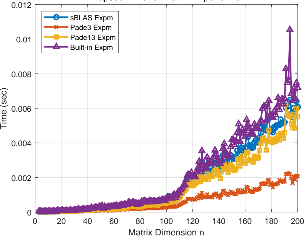
Elapsed Time for Matrix Exponential
