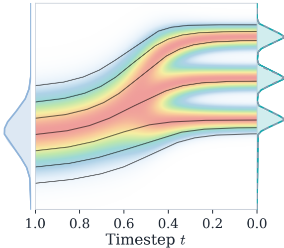
(a) PF-ODE (no rescaling)
