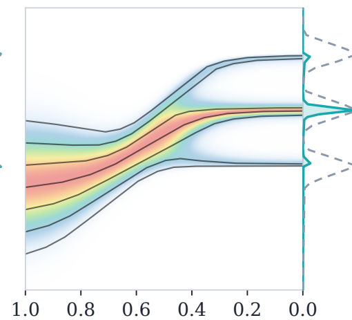
(c) TSR ( k=2, \sigma=10 )
