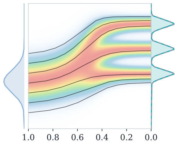
(a) PF-ODE (no rescaling)
