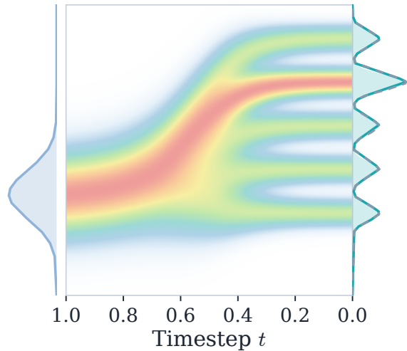
(a) PF-ODE (no rescaling)
