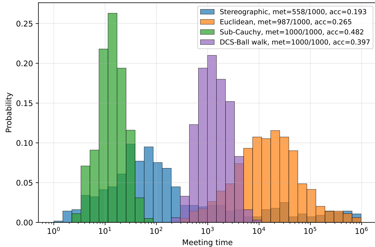
Finite meeting times (met pairs only)
