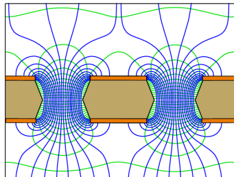
Fig. 2: Electric field lines in a GEM detector
