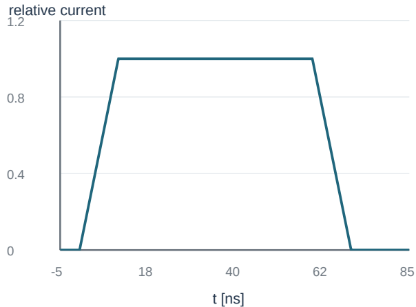
60 ns arrival spread + 10 ns response
