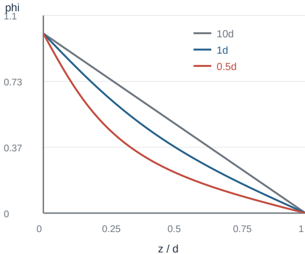
Central axis: weighting potential
