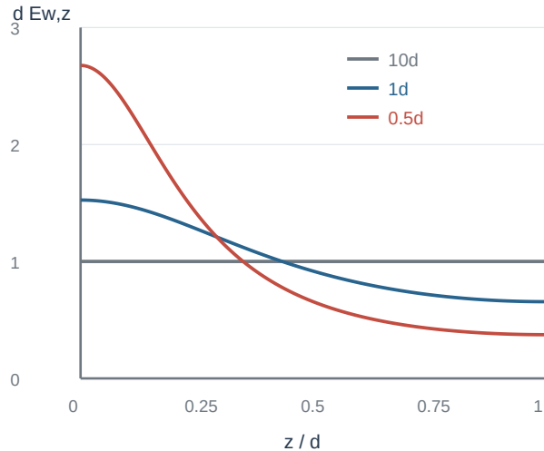
Central axis: weighting field
