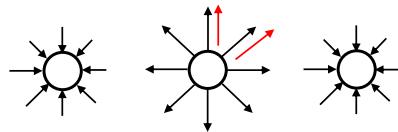
Weighting field of the signal wire
