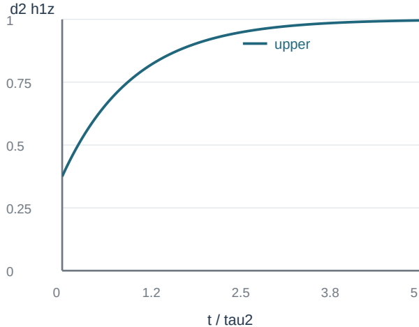
Step response: upper layer
