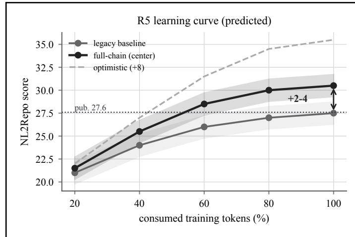
Figure 10: Planning prior (predicted, not measured) . R5: score versus consumed-token learning curve at fixed 20/40/60/80/100% checkpoints. Predicted qualitative shape: near-overlapping early, a smooth positive gap that may saturate, with a final +2–4 center effect (red) and a +8 optimistic scenario (soft-red dashed). Success gate: fixed final-checkpoint effect with seed-aware CI excluding zero. A jump only at the last checkpoint suggests noise/selection; an advantage confined to low budgets is data efficiency, not higher final capability.
