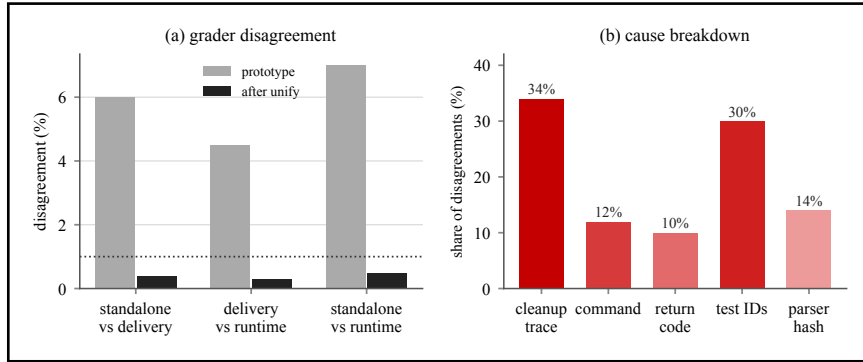
Figure 14: Planning prior (predicted, not measured) . A4: differential grader parity across standalone replay, delivery grade.py, and runtime evaluator. (a) predicted pairwise disagreement falls from a 1–10% prototype range to 0–0.5% after unification; (b) predicted cause breakdown, dominated by cleanup-trace and test-ID differences (a same score with different IDs still counts as disagreement). Success gate: canonical controls at exact parity and aggregate disagreement upper bound below 1%. Residual cleanup/parser disagreement means validation is not the deployed judge.
