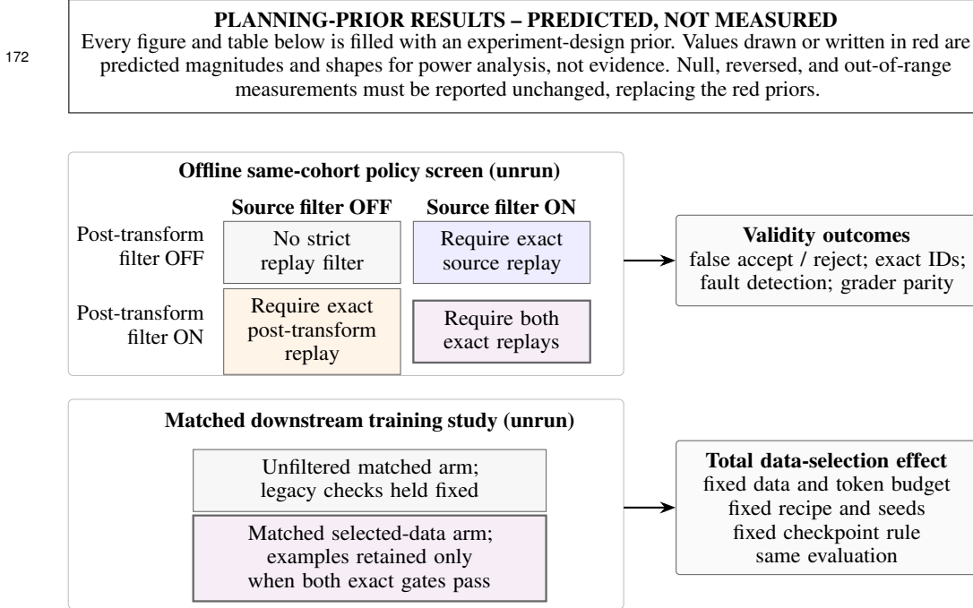
Figure 6: Pre-specified validation. The 2 \times 2 settings are policy filters on one offline cohort, not per-task pass labels. A separate matched two-arm training study estimates only the total effect of requiring both exact gates under fixed data volume and recipe. No result is reported before manifests and runs exist.
