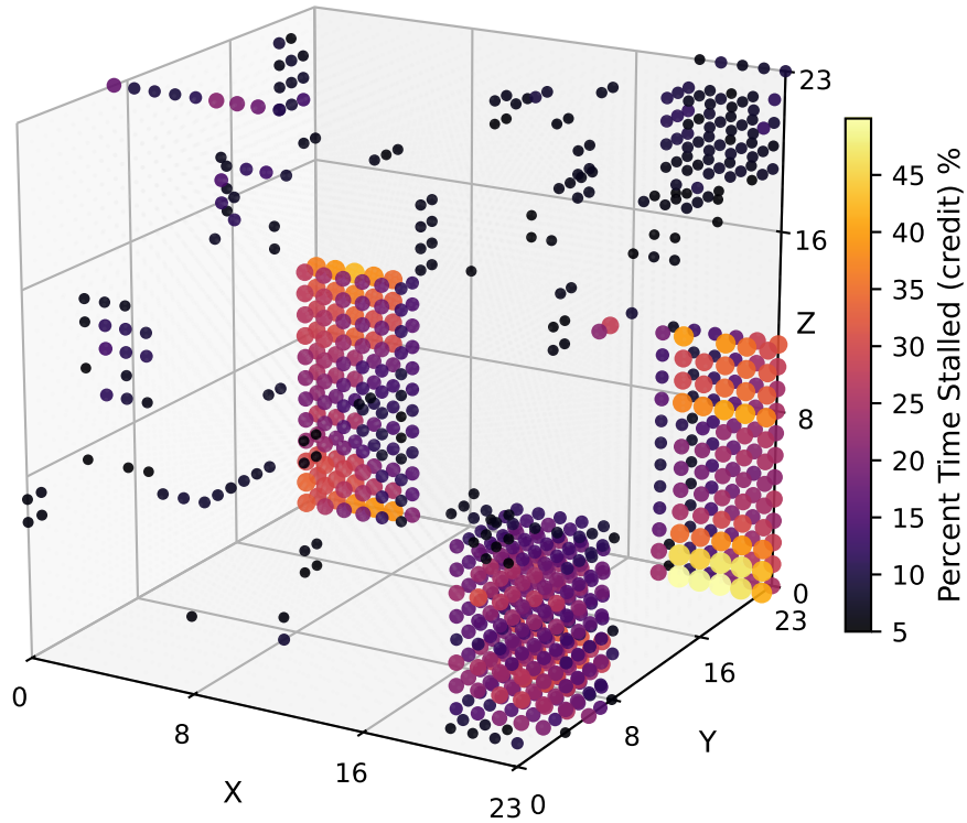
(c) Region growth, floor 15
