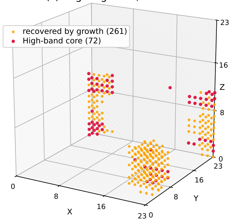
(c) Region growth, floor 15
