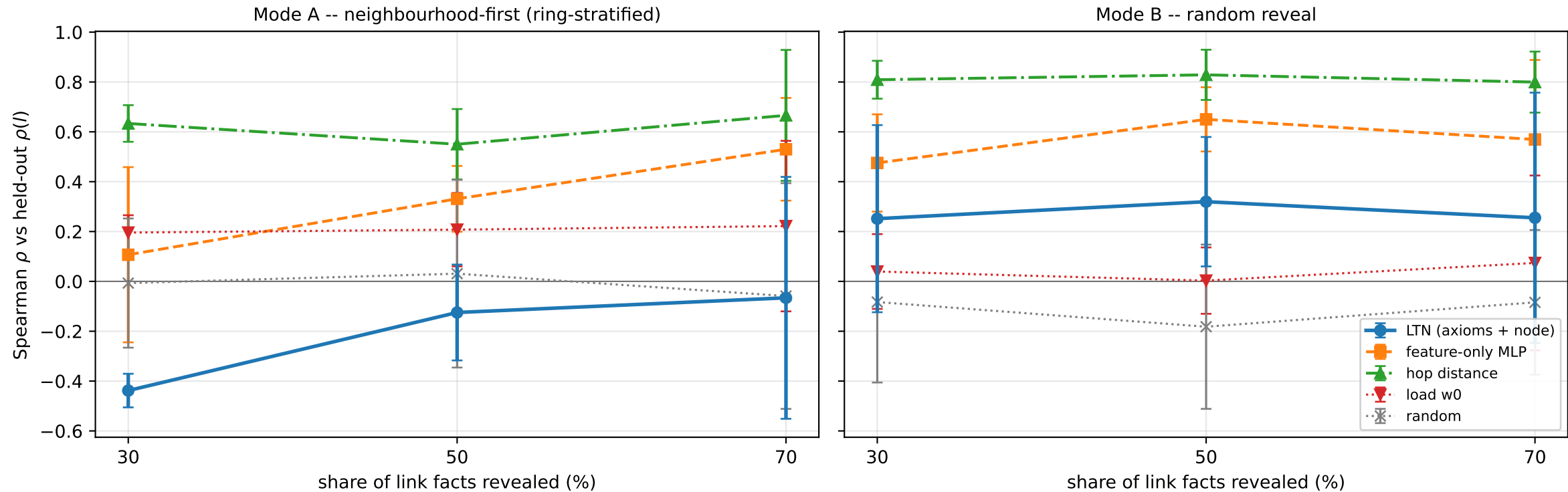
Held-out link inference after Link_Down(Berlin, Hamburg), 10 seeds (mean \pm std)
