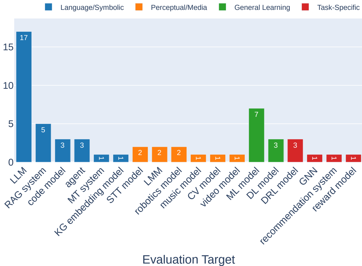
Number of Evaluation Harnesses
