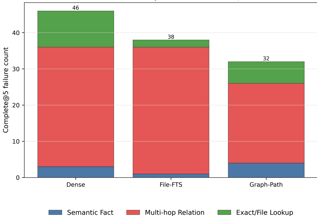
Failure Cases by Baseline and Task @5
