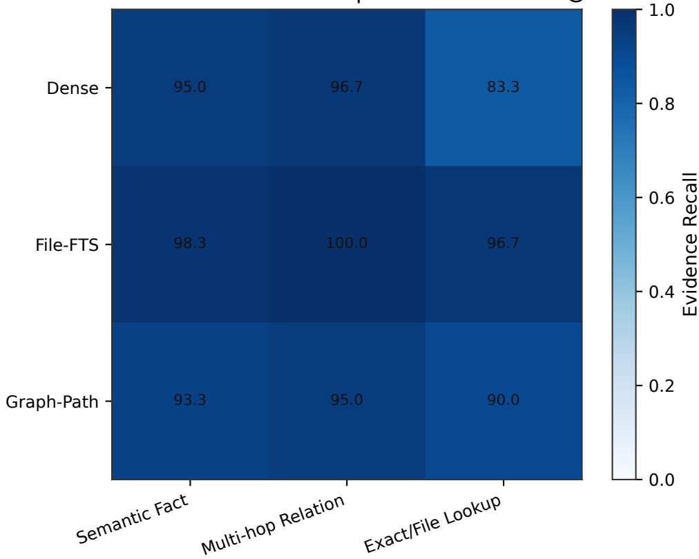
Task x Baseline Heatmap: Evidence Recall @5
