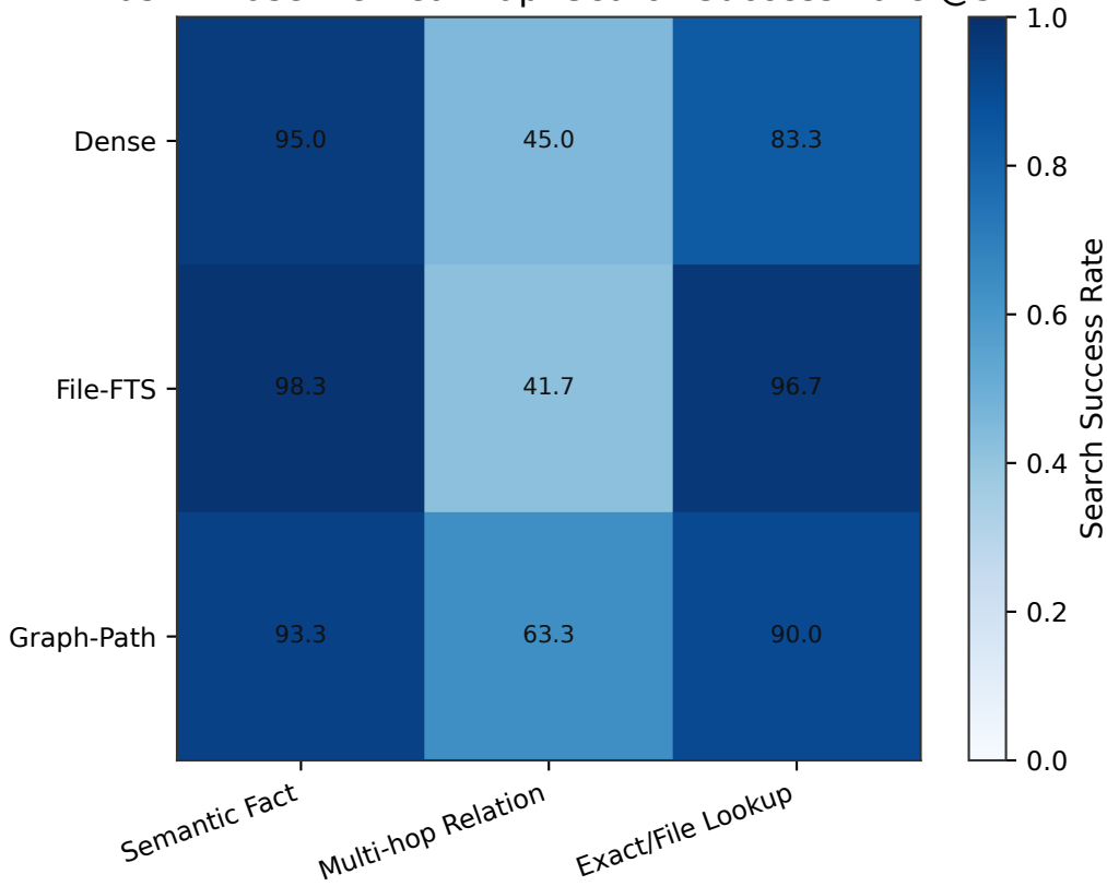
Task x Baseline Heatmap: Search Success Rate @5
