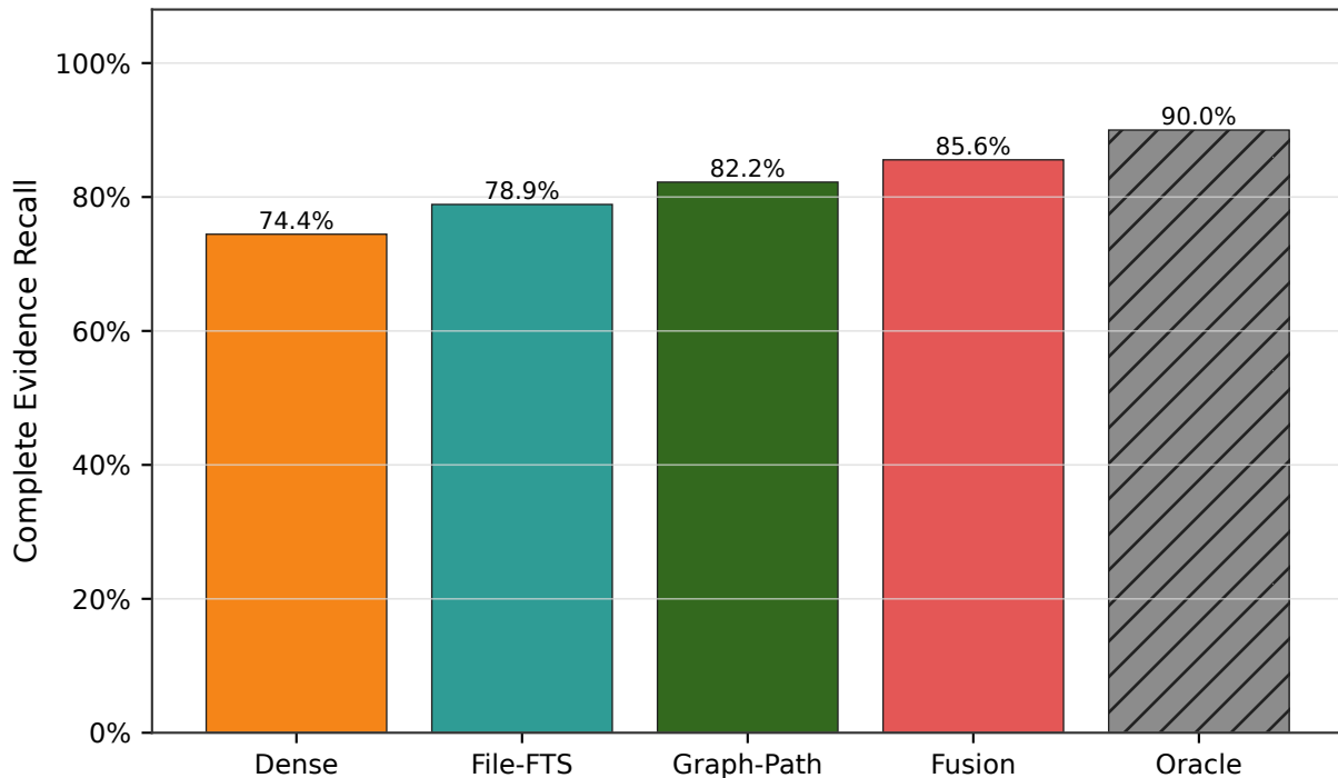
Overall @5: Complete Evidence Recall
