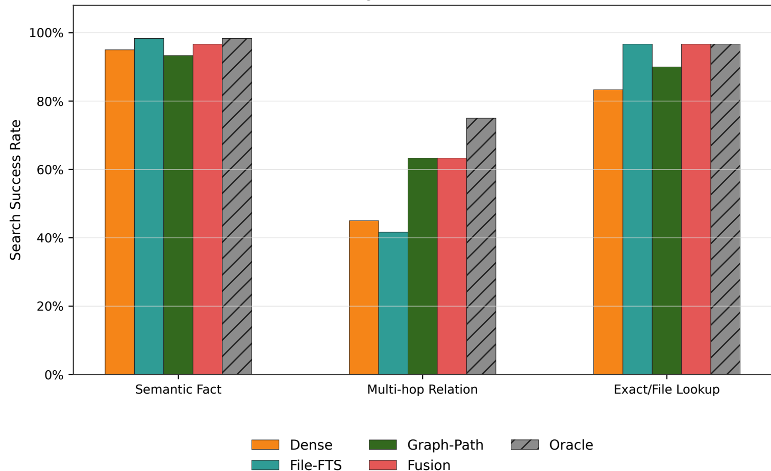
Task-wise @5: Search Success Rate
