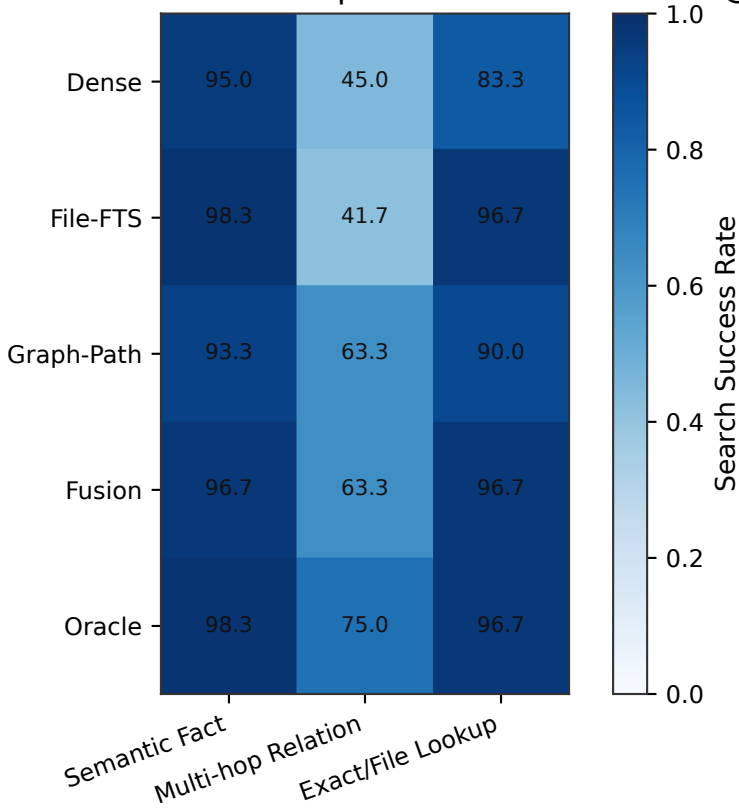
Task x Baseline Heatmap: Search Success Rate @5
