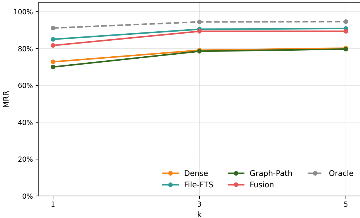
@k Sensitivity: MRR
