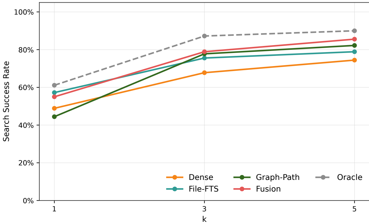
@k Sensitivity: Search Success Rate
