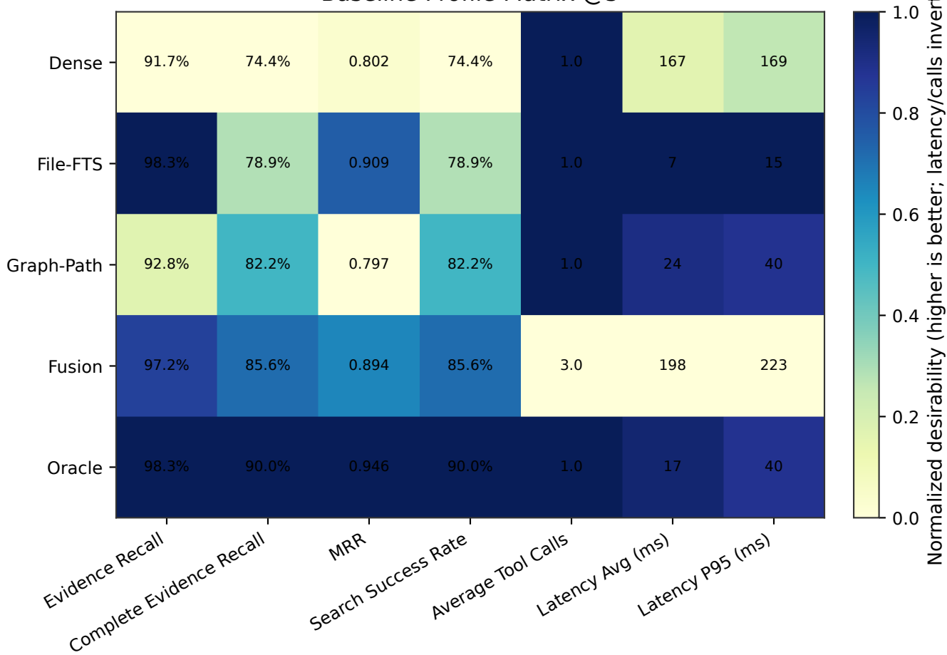
Baseline Profile Matrix @5
