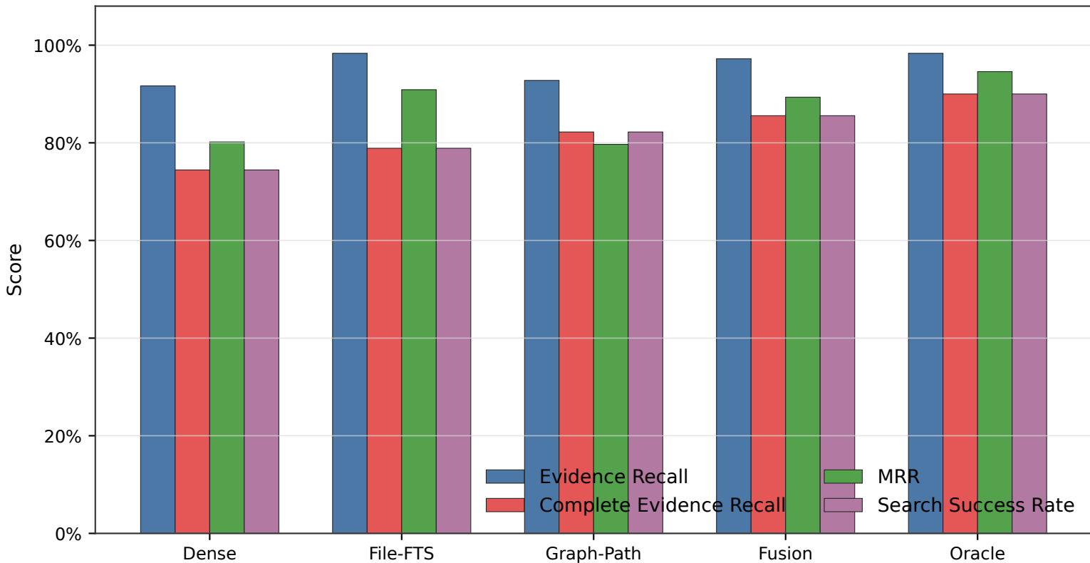
Overall @5: Quality Metrics by Baseline
