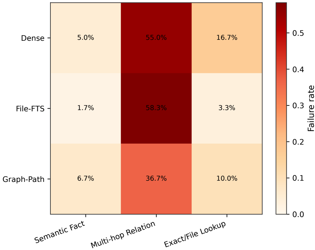
Complete@5 Failure Rate by Task
