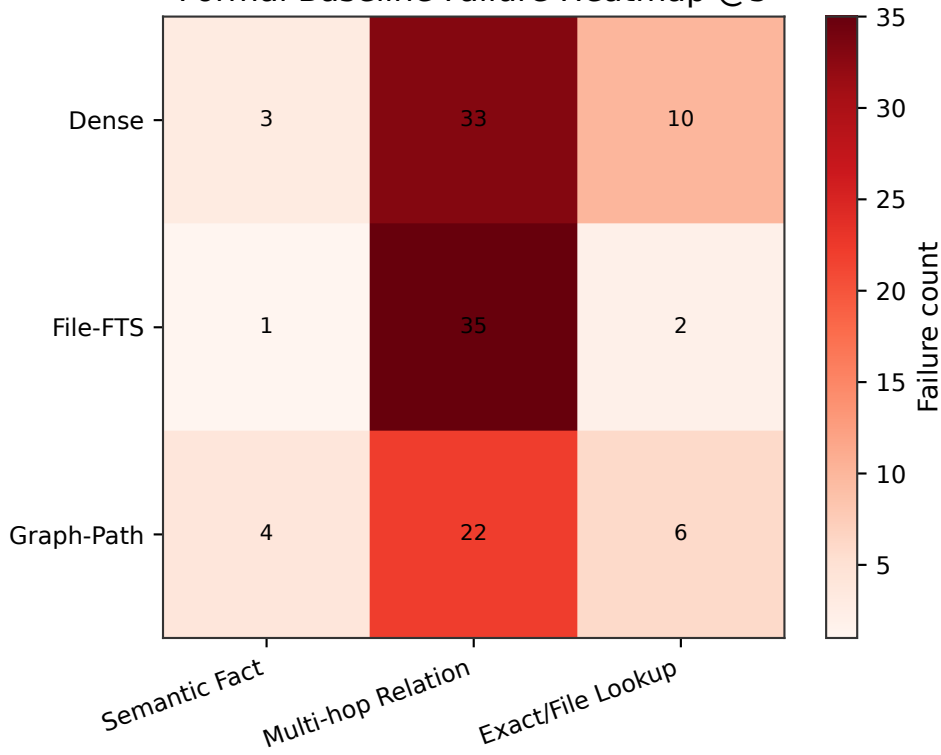
Formal Baseline Failure Heatmap @5
