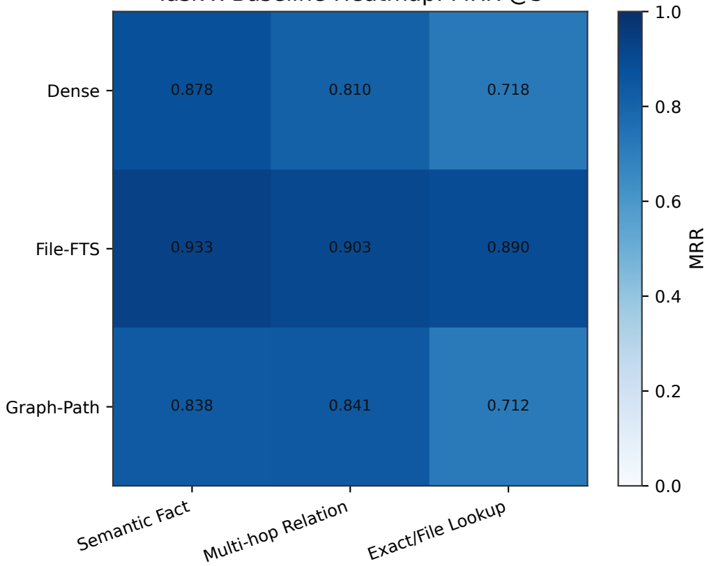
Task x Baseline Heatmap: MRR @5
