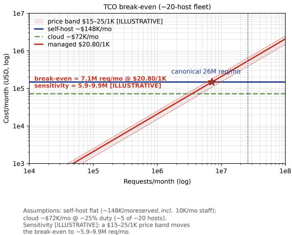
FIGURE 16.1: TCO break-even: self-hosted vs managed API [ILLUSTRATIVE][DERIVED]
