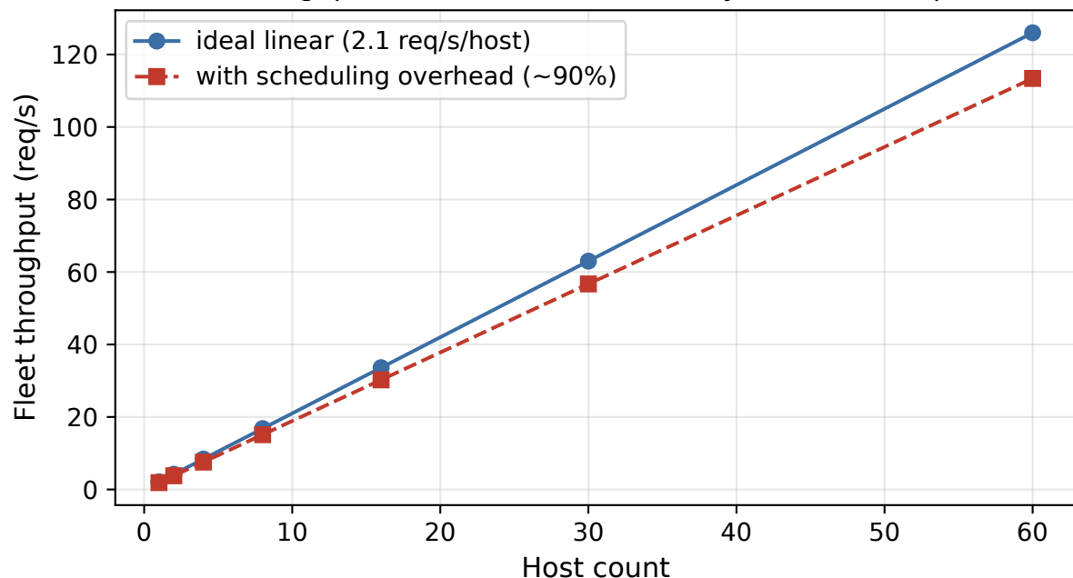
Fleet throughput vs host count (KV/latency bound 2.1 req/s/host)
