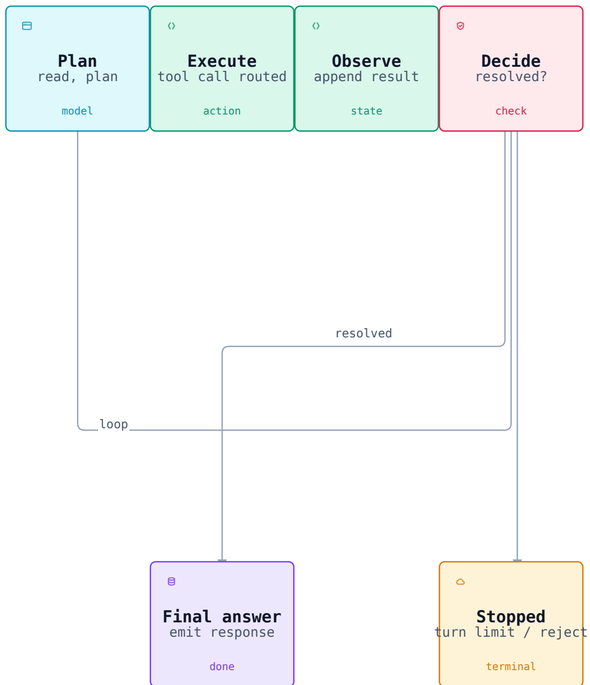
FIGURE 19.1: The agent loop as a four-state state machine (Plan, Execute, Observe, Decide) with a loop-back to Plan and the terminal outcomes final answer and stopped [ILLUSTRATIVE conceptual]
