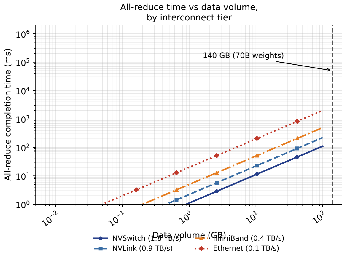
FIGURE 9.1: All-reduce time vs data volume, by interconnect tier [1P][DERIVED]
