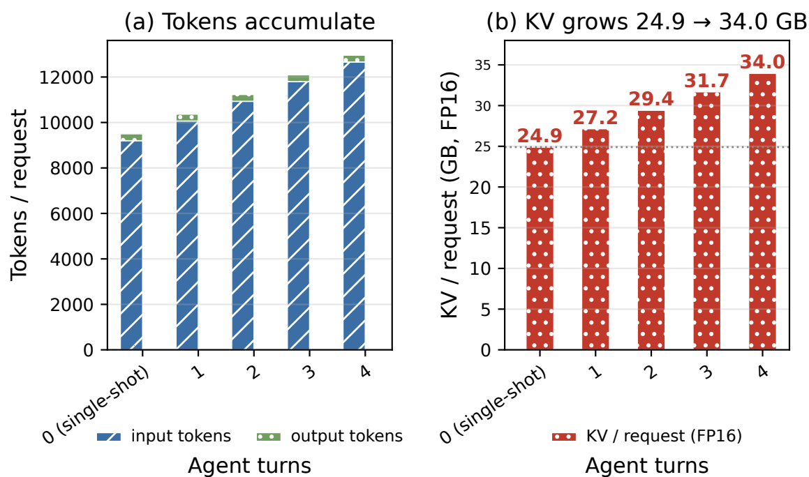
FIGURE 19.2: Input/output tokens and KV cache per request across agent turns ( I_0 + T \cdot \delta + T \cdot \gamma ; 9,200 + 800 + 65 per turn), FP16 KV rising from 24.9 GB single-shot to 34.0 GB at 4 turns. This chart quantifies the growth — the total token and KV numbers as turns accumulate. (Companion Fig 19.3 shows the mechanism of why it grows.) [DERIVED: Ch19 §3 arithmetic]
