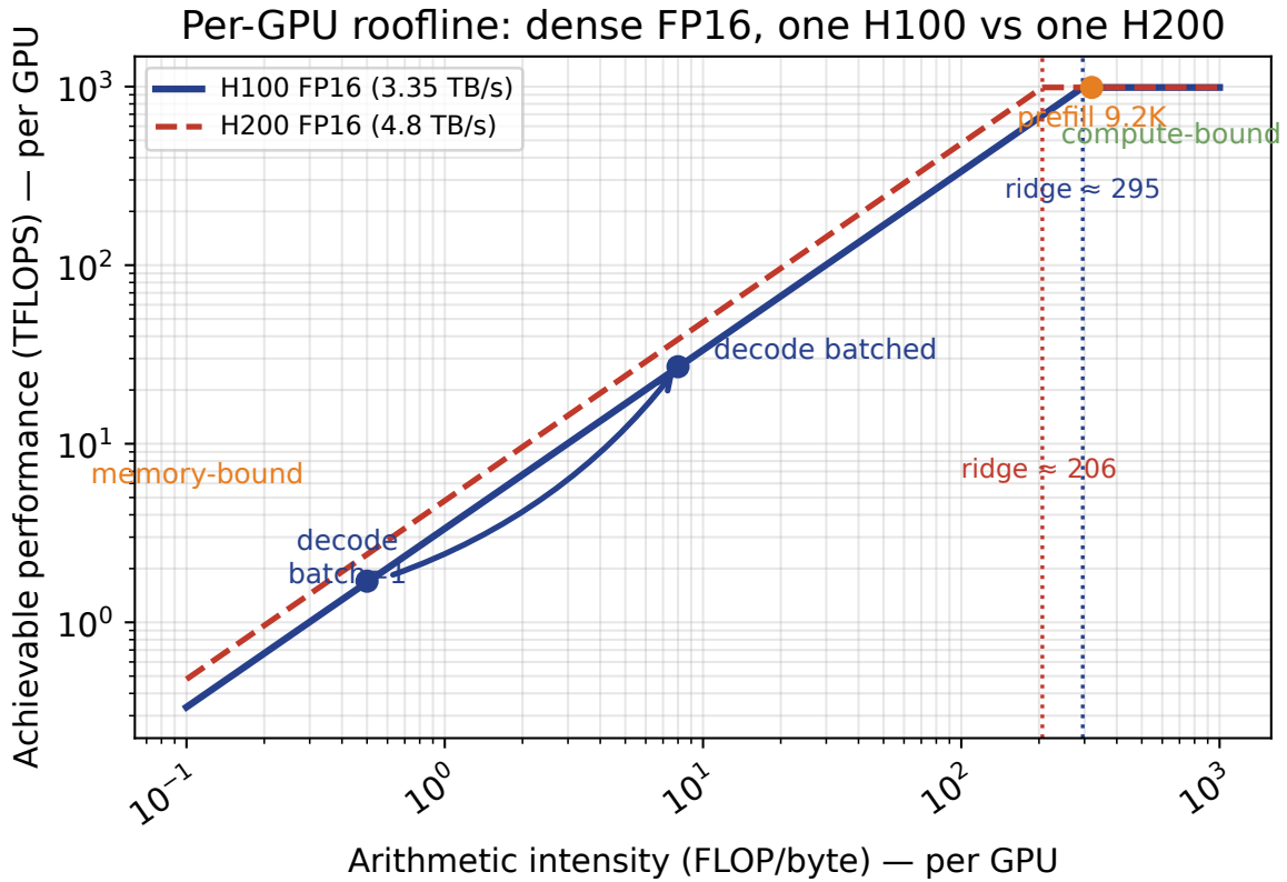
FIGURE 8.2: Per-GPU roofline for dense FP16, one H100 vs one H200 (a per-GPU chart, not a host-level one). Compute ceiling and HBM bandwidth are single-GPU quantities here (989 TFLOPS, 3.35 / 4.8 TB/s), so the ridge point and the memory-bound slope are per-GPU. Prefill (9.2K input) sits to the right of the ridge, on the compute-bound plateau; decode (batch=1) sits to the left, on the memory-bound slope, and continuous batching climbs the slope as batch grows. The ridge classification (compute- vs memory-bound) is unchanged by ideal N-way replication because both peak FLOP/s and HBM bandwidth scale with GPU count; host-level attainable performance additionally depends on sharding and communication. [DERIVED from 1P: vendor datasheet]
