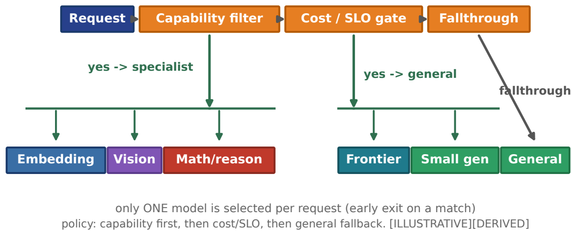
FIGURE 18.1: Model-routing decision tree: capability filter → cost/latency gate → fallthrough, with the specialist, general and fallback model families as leaves [ILLUSTRATIVE conceptual]
