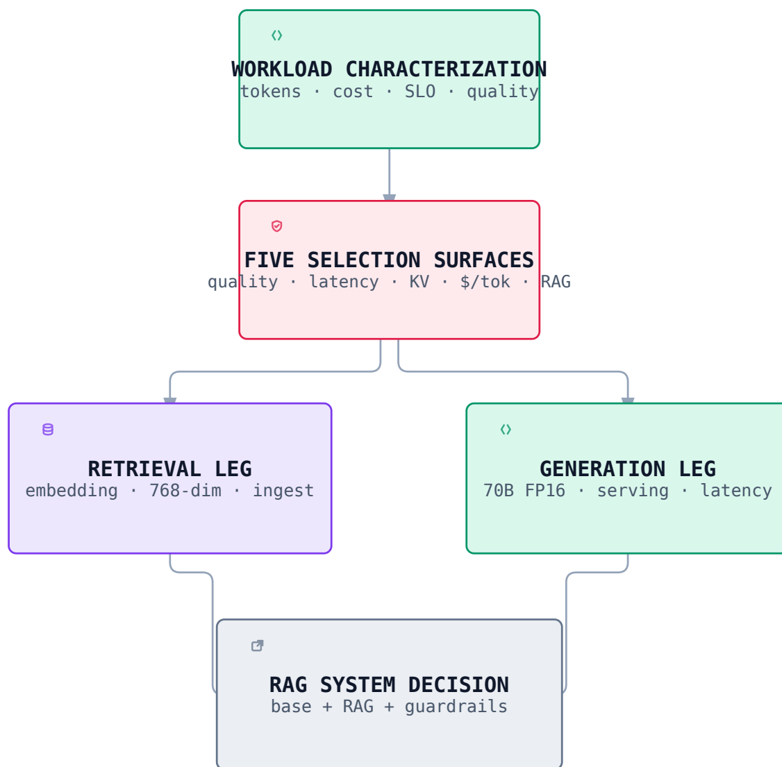
FIGURE 5.1: Model selection for RAG: workload → five selection surfaces → two legs (retrieval/embedding, generation/70B) → the system decision [ILLUSTRATIVE conceptual]
