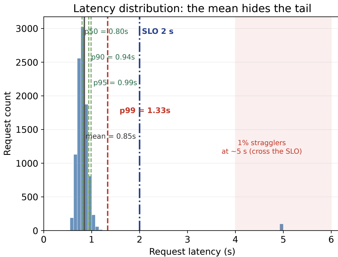
FIGURE 6.2: Request-latency distribution: p50/p90/p95/p99 and the mean
