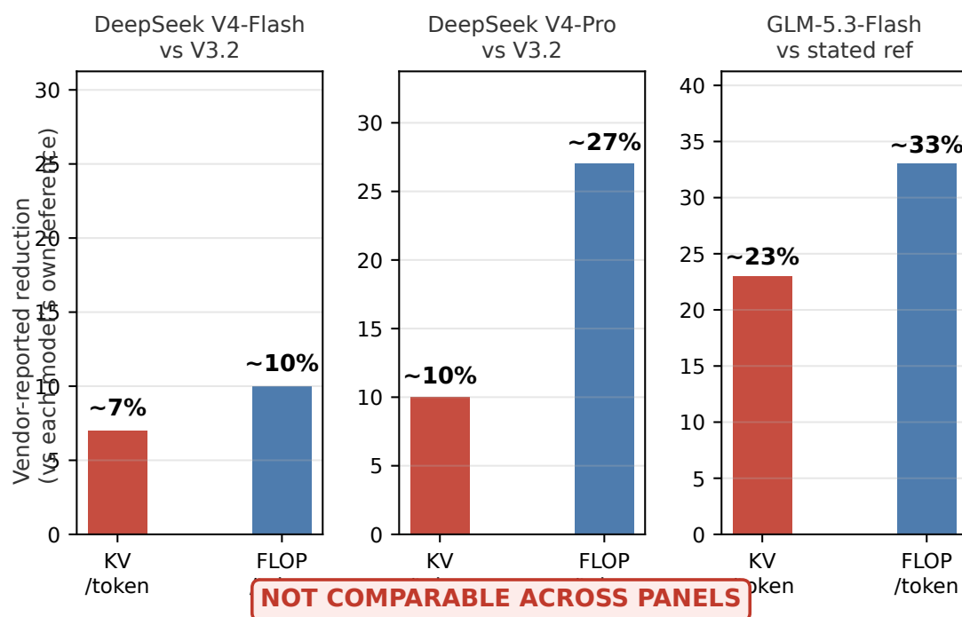
FIGURE A.2: Vendor-reported KV/FLOP reduction relative to each model's stated predecessor/reference, not a cross-model baseline [DERIVED from 1P claims: arXiv 2606.19348; HF zai-org]
