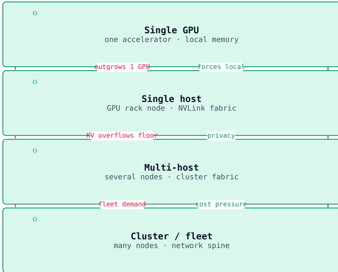
FIGURE 13.1: The reference-architecture ladder and its escalation triggers [ILLUSTRATIVE conceptual]
