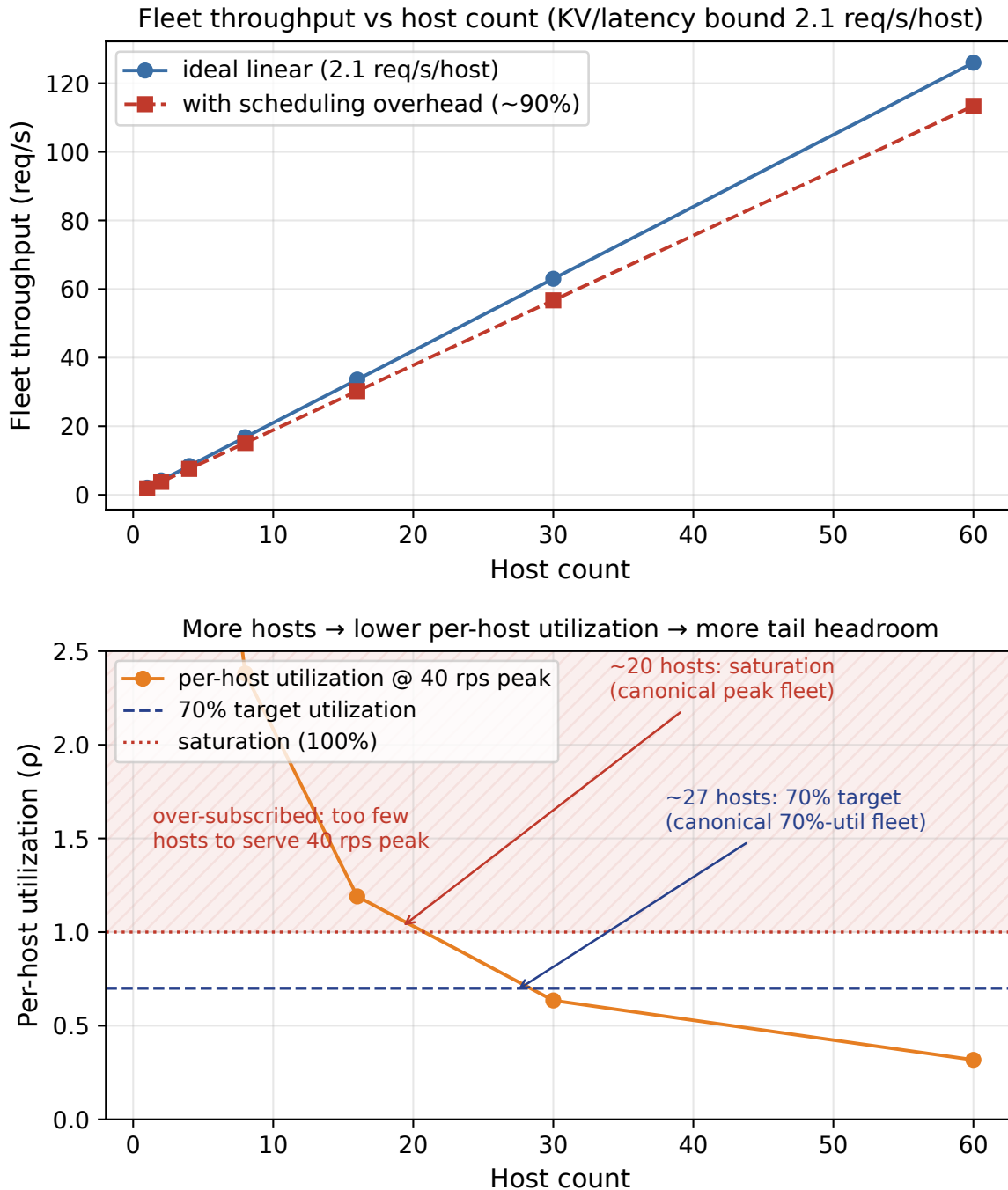
FIGURE 20.1: Fleet throughput, and per-host utilization, vs. host count at the canonical peak load (40 rps). Top panel: throughput against host count from the KV/latency bound ( \sim 2.1 req/s/host), with a \sim 90\% scheduling-overhead line. Bottom panel: per-host utilization at the canonical 40 rps peak. This is the honest quantity for the tail: p99 is driven by per-host utilization, not by host count alone . Adding hosts lowers per-host utilization (more headroom) hence lowers the expected tail; the 70%-utilization and 100%-saturation reference lines show the provisioning target. The tail also depends on the arrival process, scheduling policy, batching, and the service-time distribution, which a provisioning model alone does not capture. [ILLUSTRATIVE][DERIVED]
