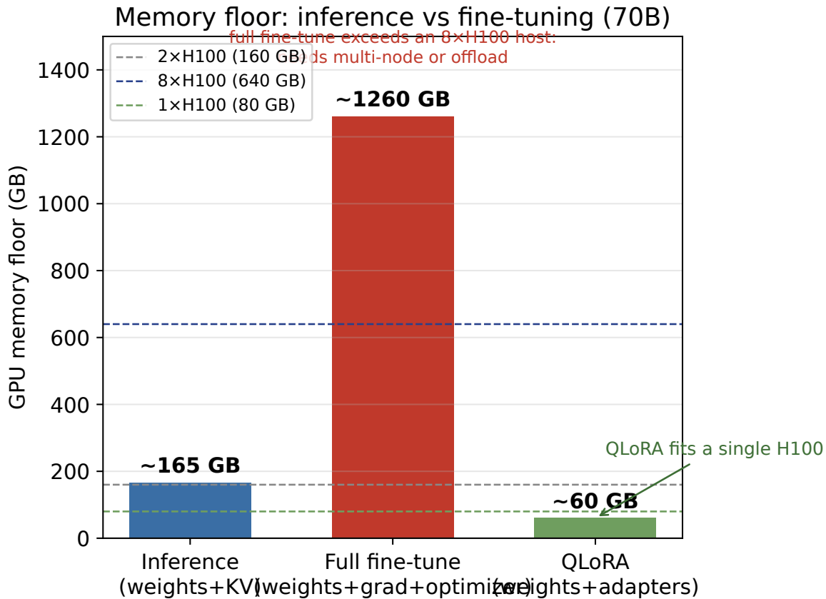
FIGURE 7.3: Inference vs fine-tuning memory floor [ILLUSTRATIVE][DERIVED]
