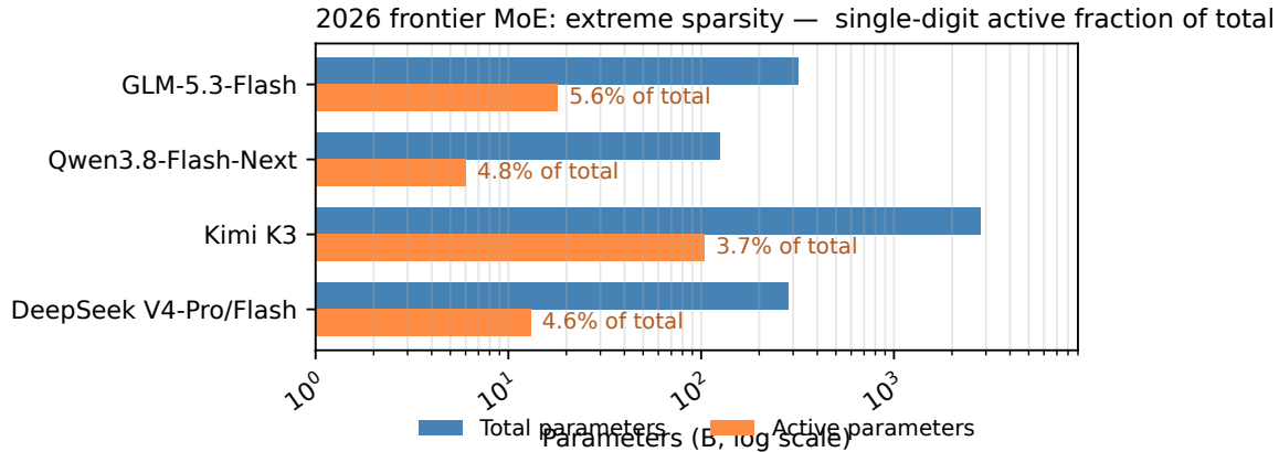
FIGURE A.1: 2026 frontier MoE extreme sparsity: four open models, total vs activated parameters, and active fraction in single digits [1P]
