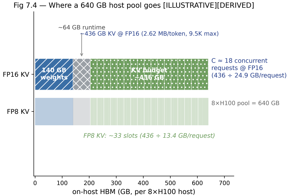
FIGURE 7.4: The concurrency budget: where a 70B host’s 640 GB pool goes. Aggregate-feasibility caveat: the 640 GB figure is an aggregate across eight 80-GB H100s, not a single freely-allotable heap. Whether a given allocation actually fits depends on tensor-parallel sharding, KV partitioning, replication, runtime layout, per-rank fragmentation, workspace requirements, and communication topology — so “total bytes < total HBM” is a necessary but not sufficient test. Per-rank fit and sharding must also be validated (Chapters 9–10). [ILLUSTRATIVE][DERIVED]
