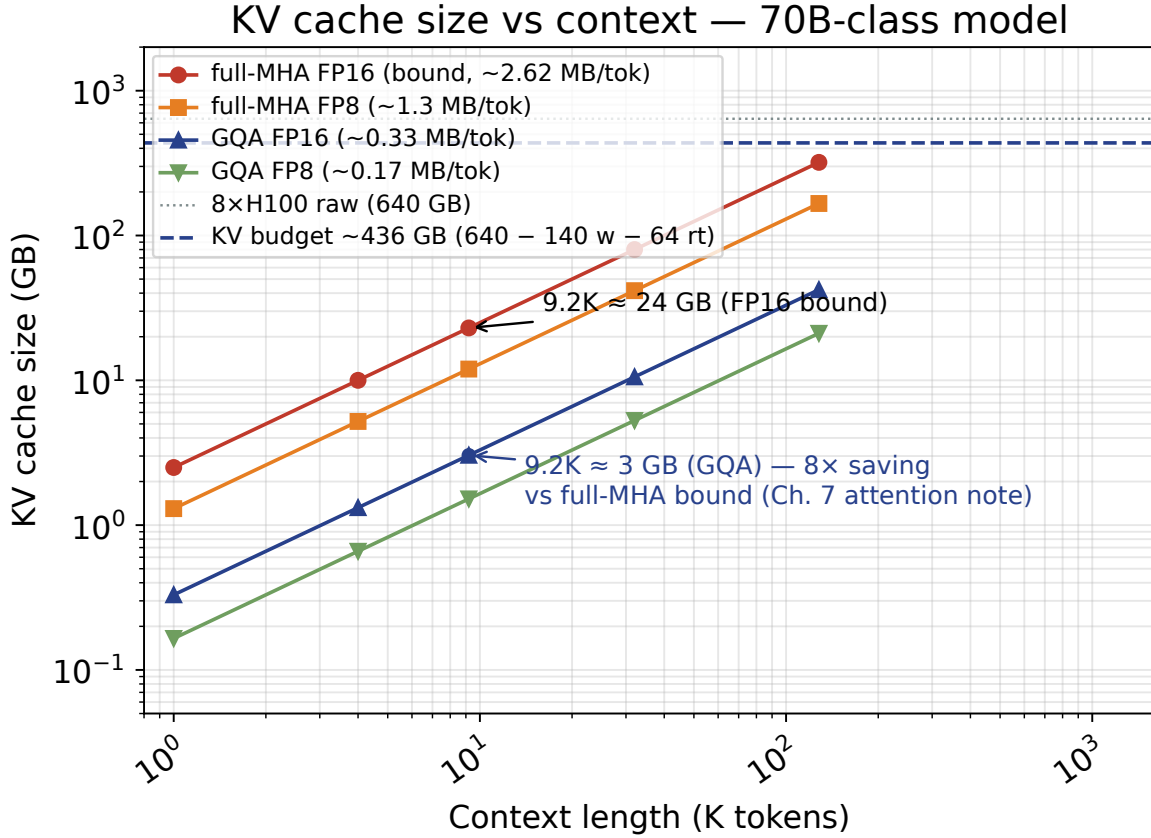
FIGURE 7.2: KV cache size vs context length for the canonical 80-layer reference geometry: full-MHA vs GQA (and FP8/8-bit). Note the broader lesson this title encodes: parameter count does not determine KV size . KV per token depends on layers \times KV-head count \times head dimension \times precision — i.e. on the attention shape , not on the number of parameters. A 70B full-MHA model and a 70B GQA model have very different KV footprints; the full-MHA curve is the conservative upper-bound teaching baseline, the GQA curve the \sim 8\times reduction. Parameter count is only a proxy for weight residency and rough dense FLOPs, never for KV footprint. [ILLUSTRATIVE][DERIVED]
