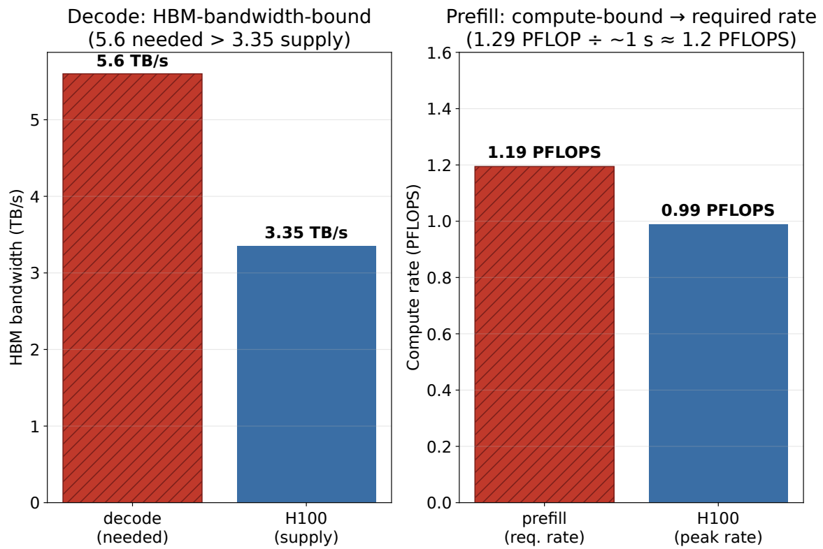
FIGURE 2.2: Decode vs prefill: bandwidth vs compute [ILLUSTRATIVE conceptual]
