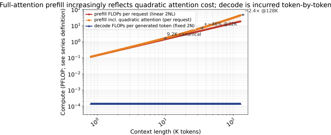
FIGURE 22.1: Full-attention prefill increasingly reflects quadratic attention cost; decode is incurred token-by-token [ILLUSTRATIVE][DERIVED]
