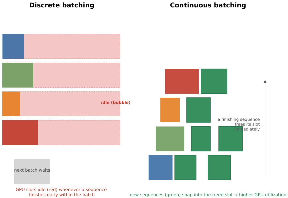
FIGURE 11.1. Fig 11.1 — Discrete vs continuous batching (Orca-style slot diagram). Discrete batching runs each batch to completion, leaving GPU slots idle as sequences finish early; continuous batching admits and evicts requests at every decode step, backfilling freed slots (ILLUSTRATIVE, after Orca, OSDI 2022)
