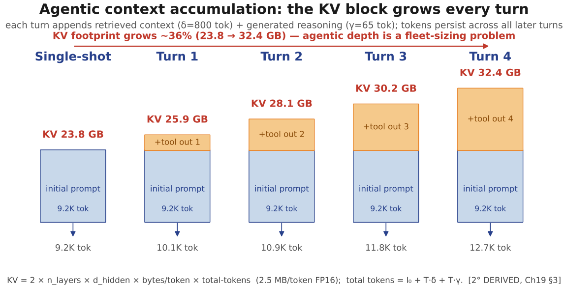
FIGURE 19.3. Fig 19.3 — The agentic context block grows every turn: initial prompt (9.2K tok) plus tool output + reasoning appended each turn, KV footprint rising 23.8 → 32.4 GB [2° DERIVED: Ch19 §3 arithmetic]
