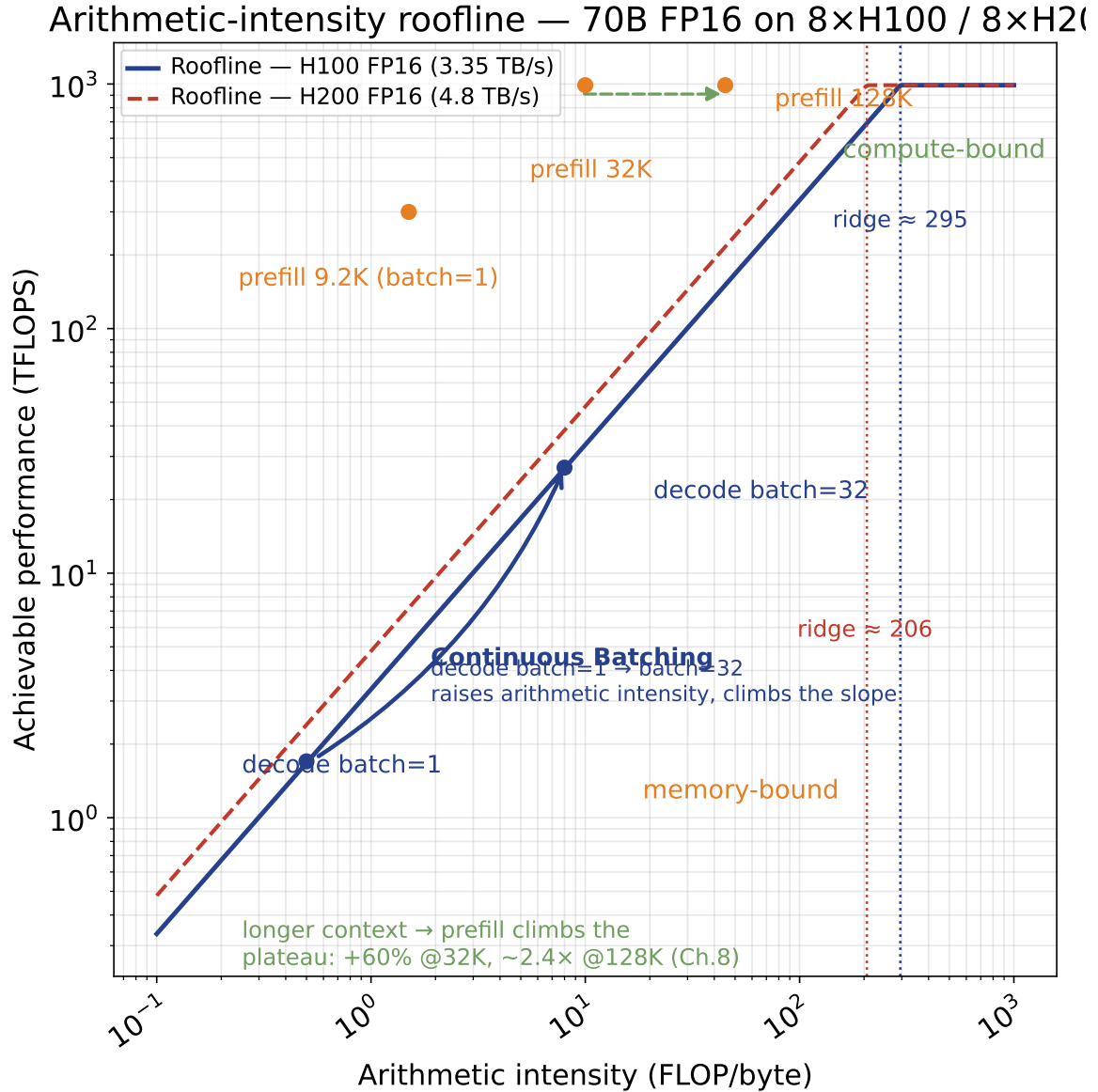
FIGURE 8.1. Fig 8.1 — Prefill above the ridge (compute-bound), decode below it (memory-bound). H100 (solid) vs H200 (dashed) ridge points from vendor datasheets (989 TFLOPS, 3.35 / 4.8 TB/s); Continuous-Batching arrow shows decode climbing the slope as batch grows [2° DERIVED] [1P: vendor datasheet]
