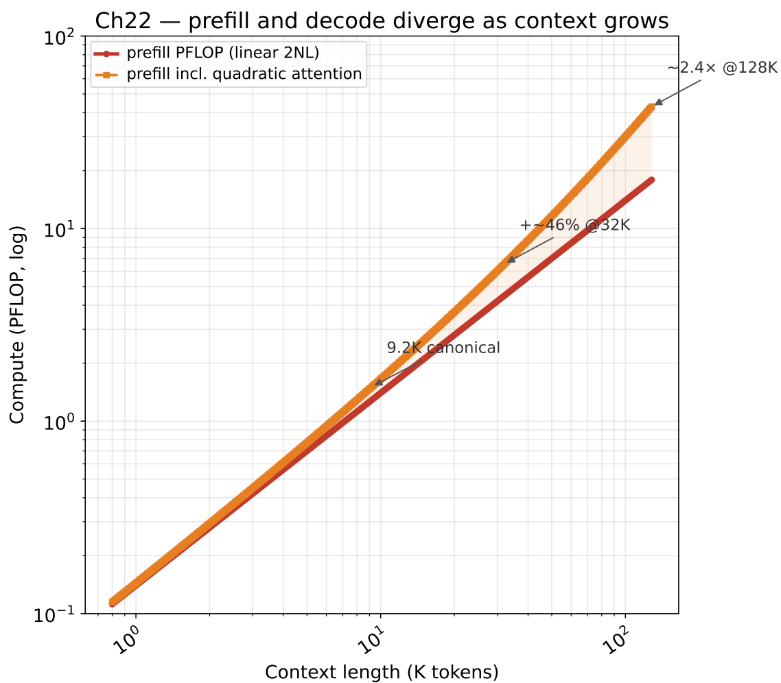
FIGURE 22.1. Fig 22.1 - Prefill vs decode bottleneck divergence [2° DERIVED]
