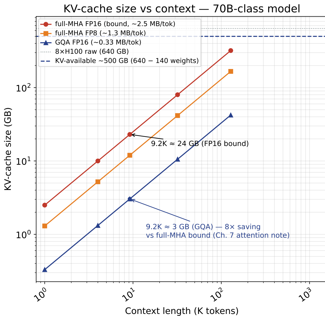
FIGURE 7.2. Fig 7.2 — KV-cache size vs context length for a 70B model [2° DERIVED]
