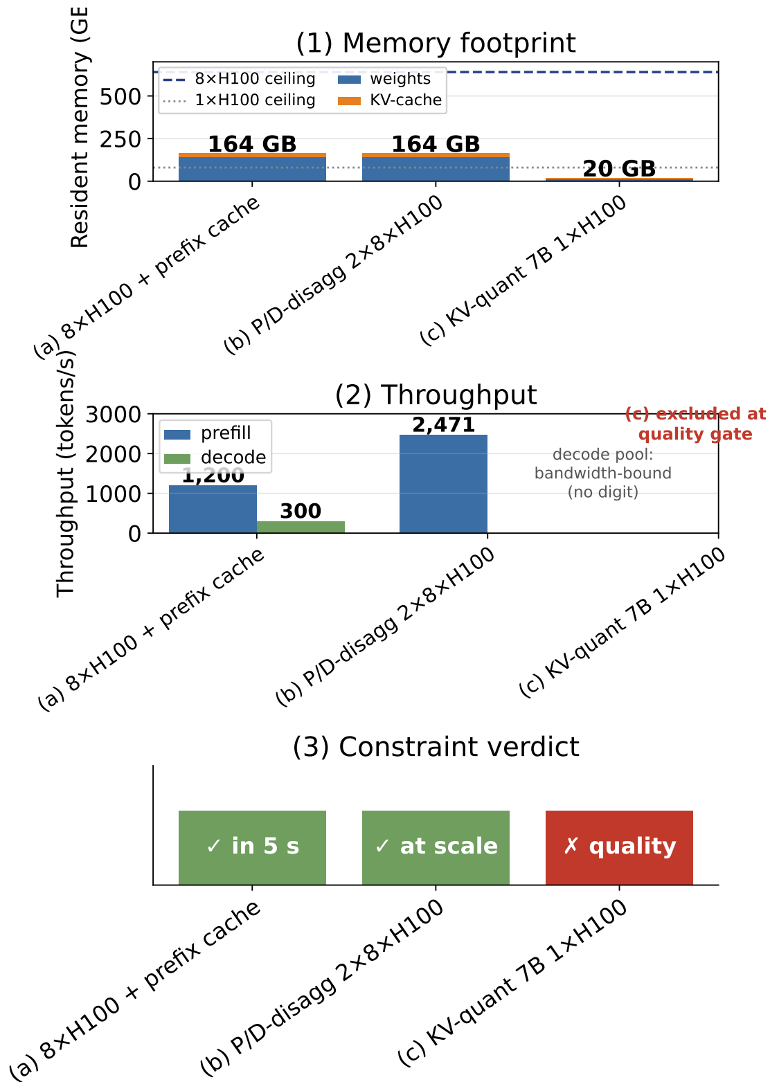
FIGURE 12.1. Fig 12.1 — Candidate architecture synthesis: three candidate architectures from the canonical enterprise-Q&A RAG workload, comparing memory residency, parallelism plan, and constraint-satisfaction outcome (memory fit, latency SLO, economics) [ILLUSTRATIVE conceptual]
