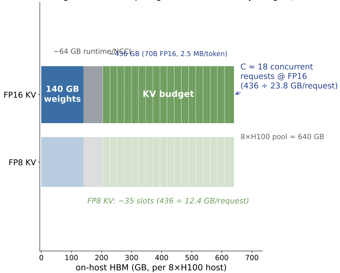
FIGURE 7.4. Fig 7.4 — The concurrency budget: where a 70B host's 640 GB pool goes [2° DERIVED]
