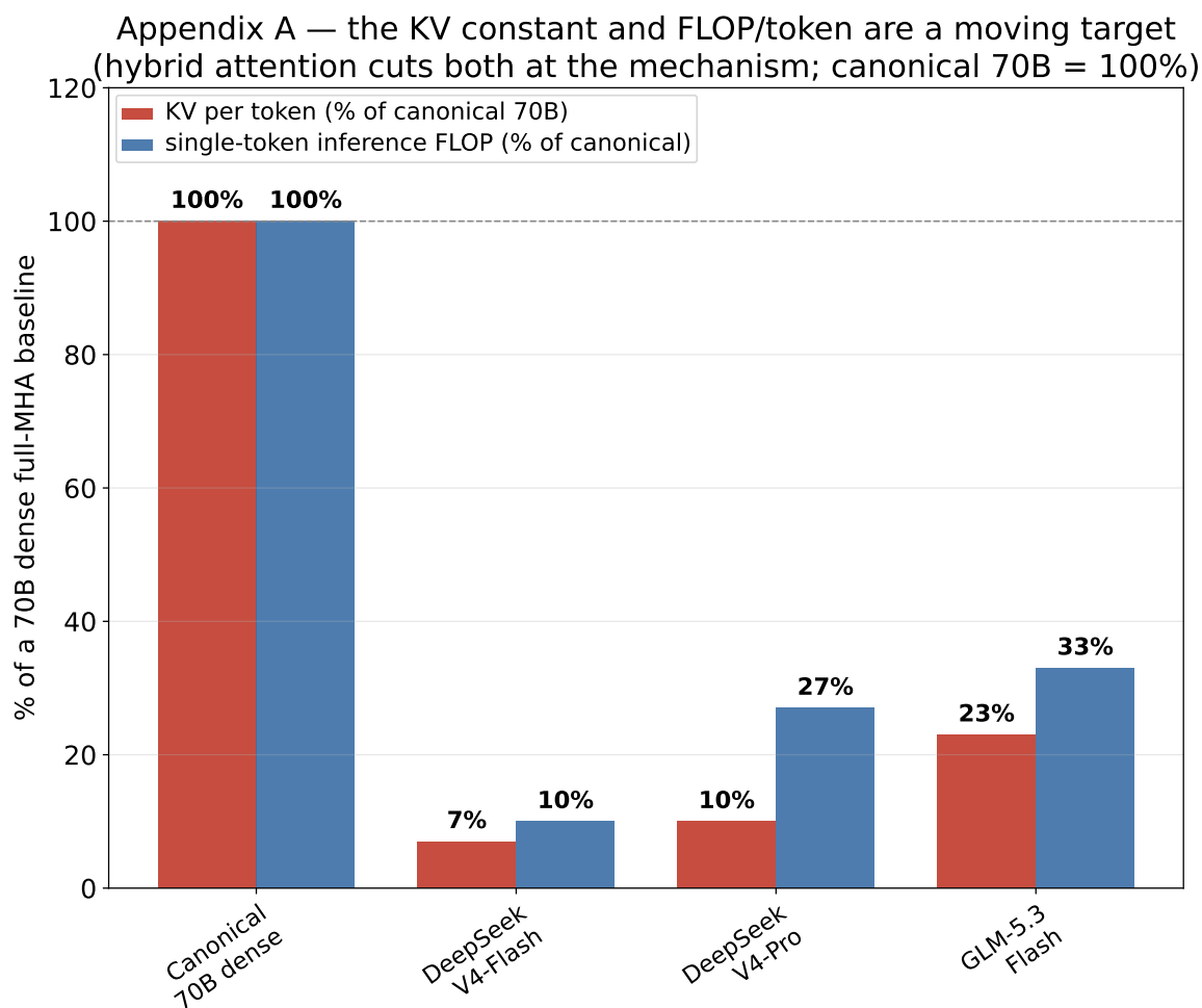
FIGURE A.2. Fig A.2 — The KV constant and FLOP/token are a moving target: hybrid attention cuts both at the mechanism. Canonical 70B dense full-MHA = 100%; DeepSeek-V4-Flash \approx 7% KV / 10% FLOP, V4-Pro \approx 10% / 27%, GLM-5.3-Flash \approx 23% KV / \sim 33% attention-compute [DERIVED from 1P claims: arXiv 2606.19348; HF zai-org]
