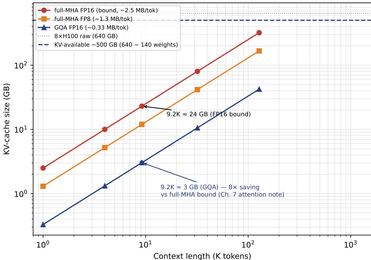
KV-cache size vs context — 70B-class model
